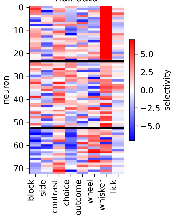
ss_z: 1.82
