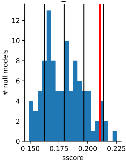
ss_z: 1.82
