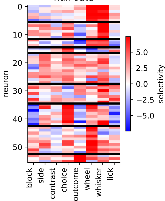
ss_z: 5.69
