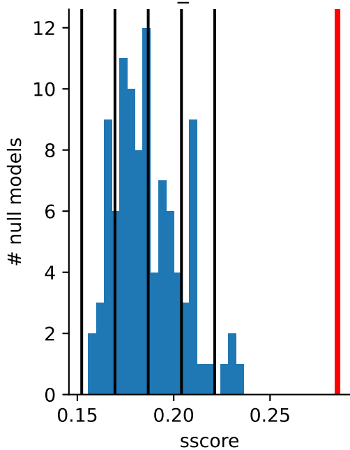
ss_z: 5.69
