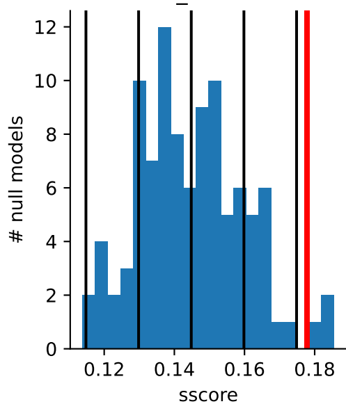
ss_z: 2.20
