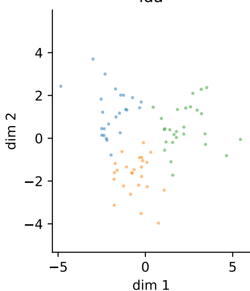
lda
