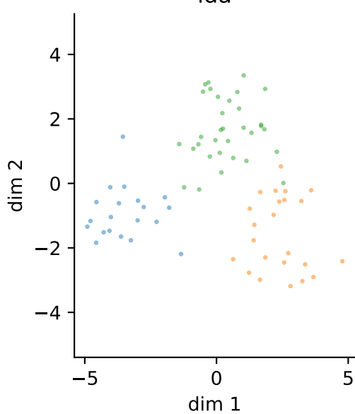
lda
