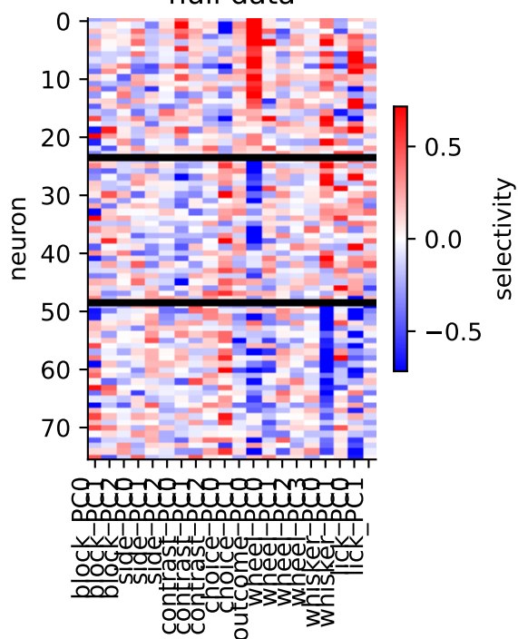
ss_z: 2.20
