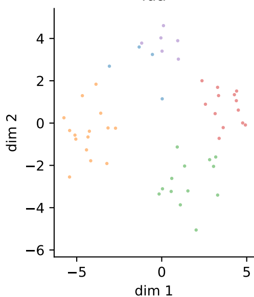
lda
