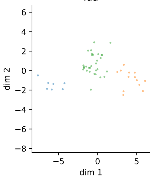
lda
