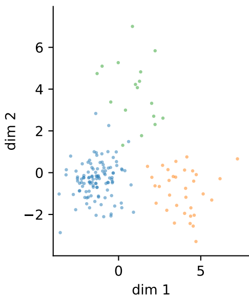
lda
