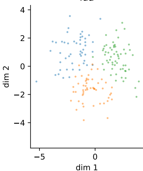
lda
