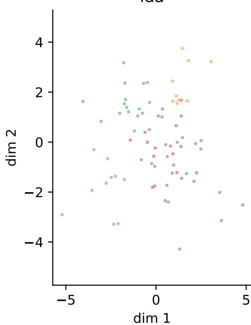
lda
