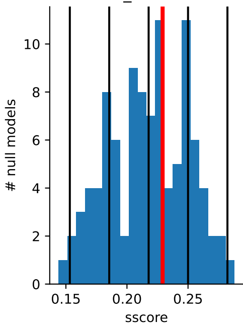
ss_z: 0.35
