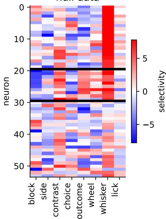
ss_z: 0.35
