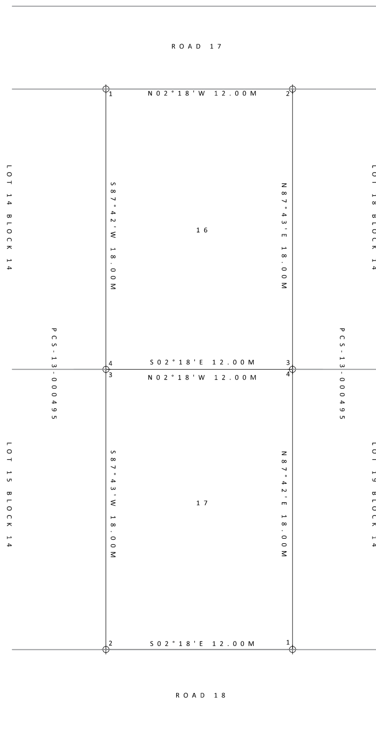
4 A-01 LOT PLAN SCALE: NTS.
