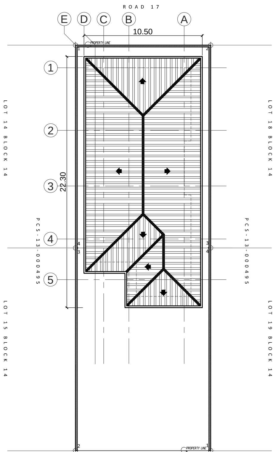
3 A-01 SITE DEVELOPMENT PLAN SCALE: 1:200 MTS.
