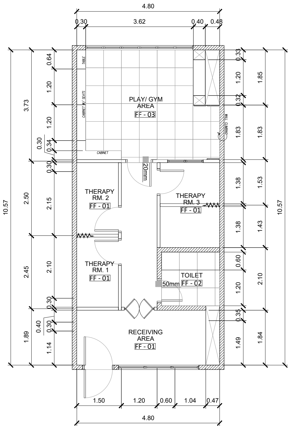
1 FLOOR FINISH LAYOUT A-02 SCALE: 1:75 MTS.
