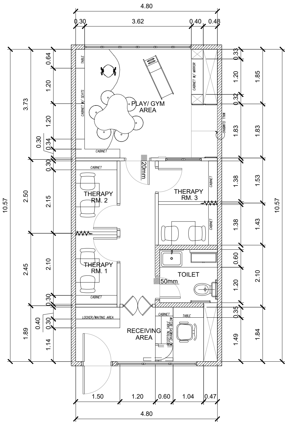
2 FURNITURE LAYOUT A-02 SCALE: 1:75 MTS.
