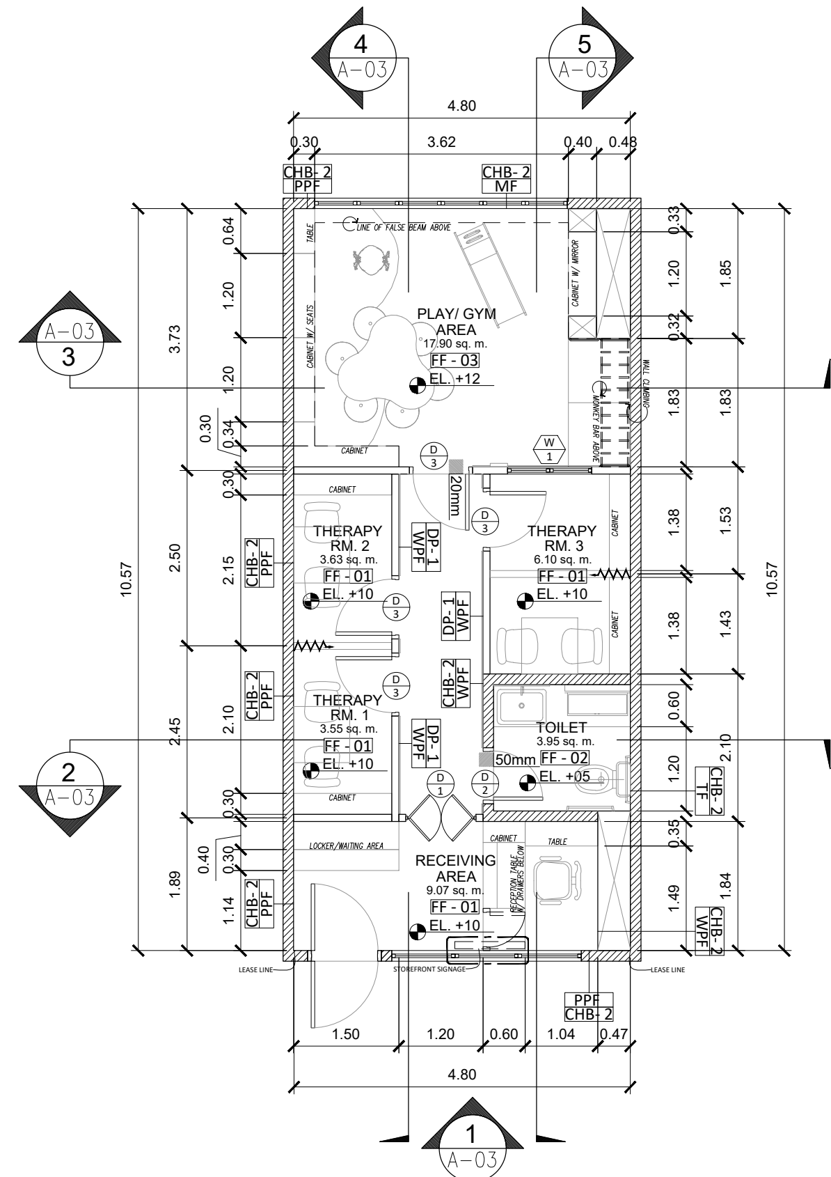
4 GROUND FLOOR PLAN A-02 SCALE: 1:75 MTS.
