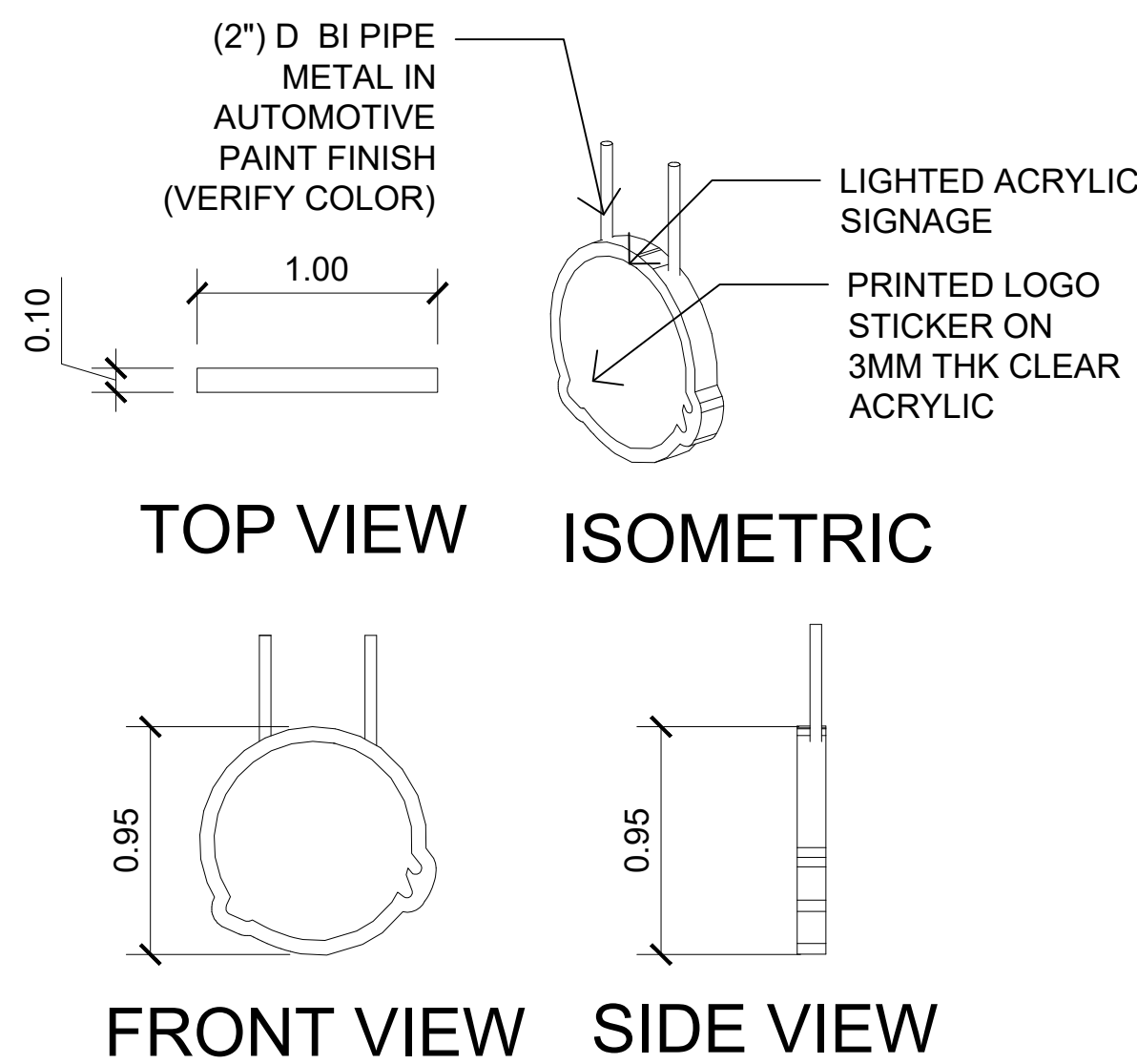
3 STOREFRONT SIGNAGE BLOW-UP DETAIL (C) A-04 SCALE: 1:30 MTS.
