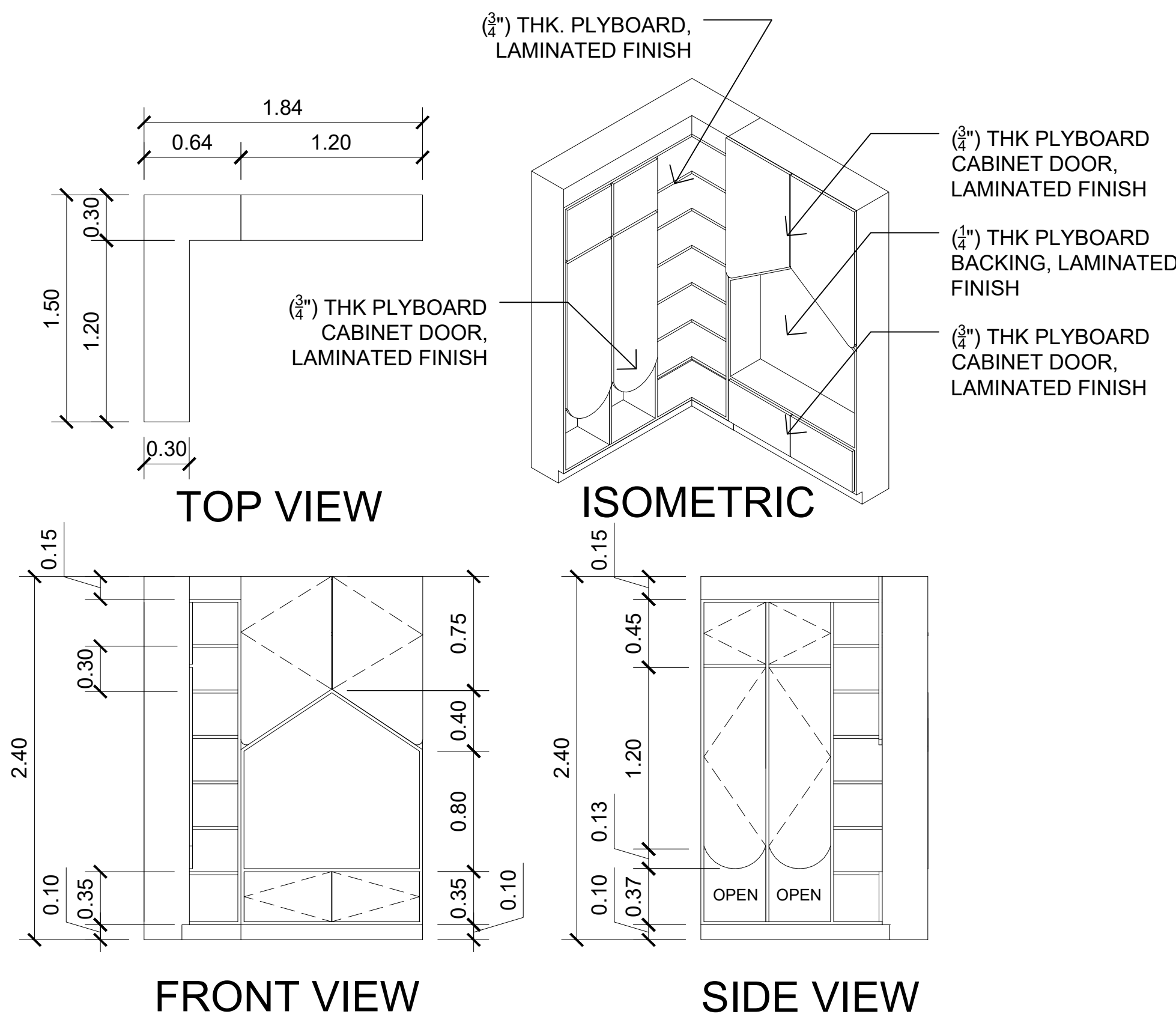
1 BLOW-UP DETAIL (A) A-04 SCALE: 1:30 MTS.
