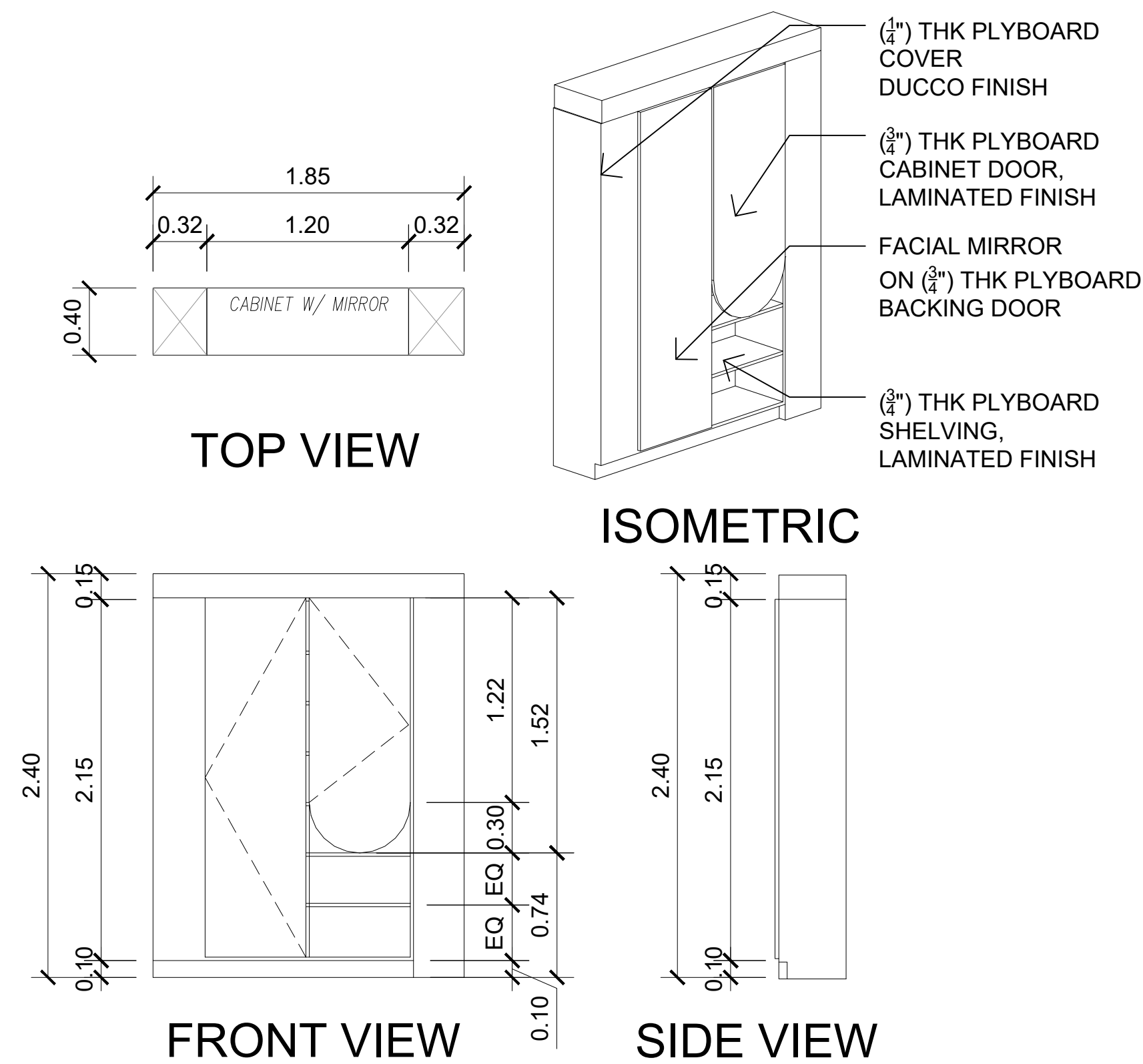
2 BLOW-UP DETAIL (B) A-04 SCALE: 1:30 MTS.
