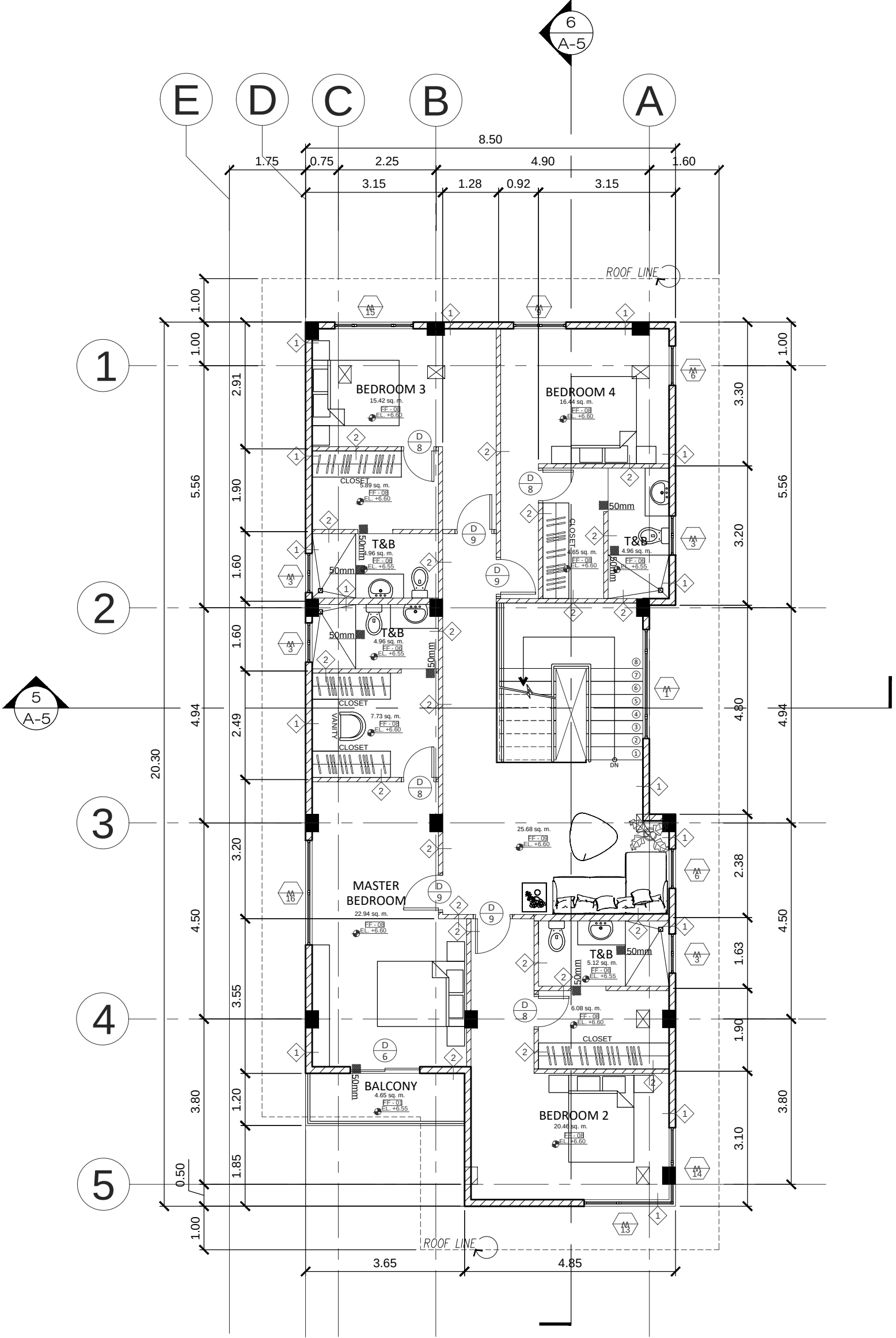
ARANETA RESIDENCE 1 THIRD FLOOR PLAN A-03 SCALE: 1:100 MTS.
