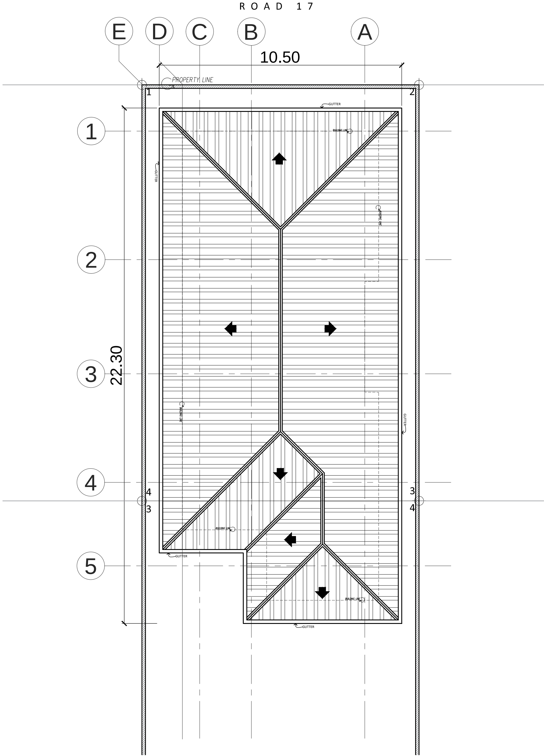
ARANETA RESIDENCE 2 ROOF PLAN A-03 SCALE: 1:100 MTS.
