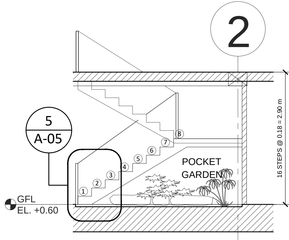
ARANETA RESIDENCE 4 STAIR DETAIL SECTION A A-05 SCALE: 1:50 MTS.
