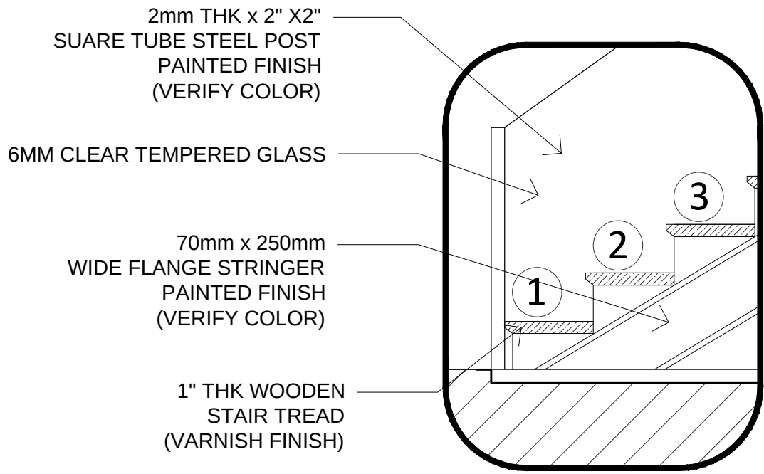
ARANETA RESIDENCE 5 STAIR DETAIL SECTION B A-05 SCALE: 1:20 MTS.
