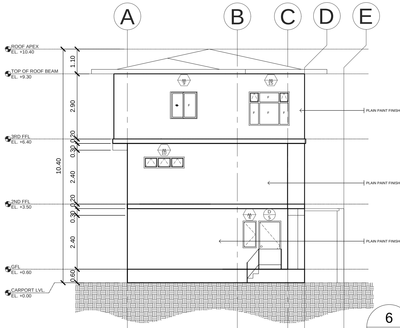
ARANETA RESIDENCE 4 RIGHT SIDE ELEVATION A-06 SCALE: 1:100 MTS
