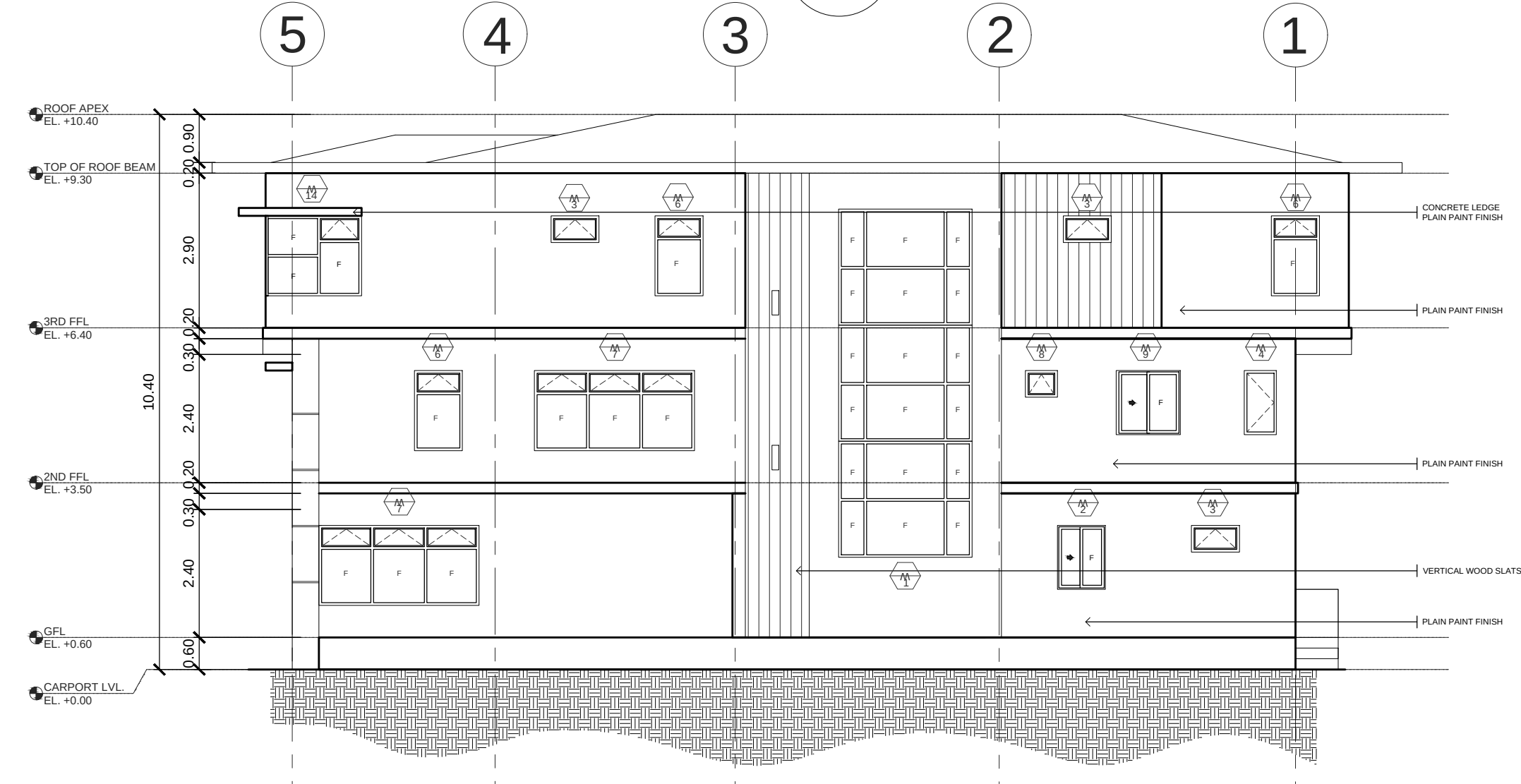
ARANETA RESIDENCE 5 LEFT SIDE ELEVATION A-06 SCALE: 1:100 MTS
