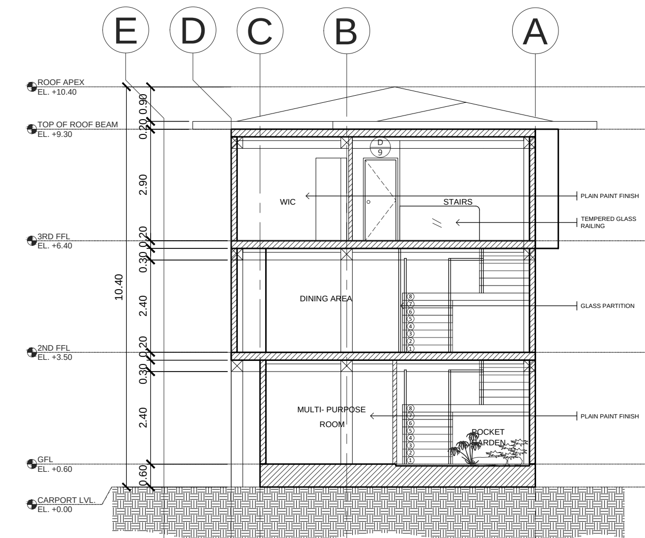
ARANETA RESIDENCE 1 CROSS SECTION A-06 SCALE: 1:100 MTS
