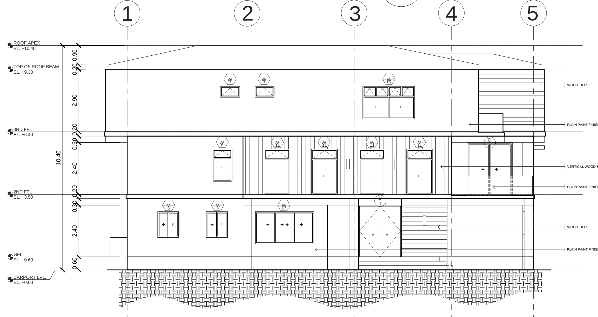
ARANETA RESIDENCE 4 RIGHT SIDE ELEVATION A-06 SCALE: 1:100 MTS
