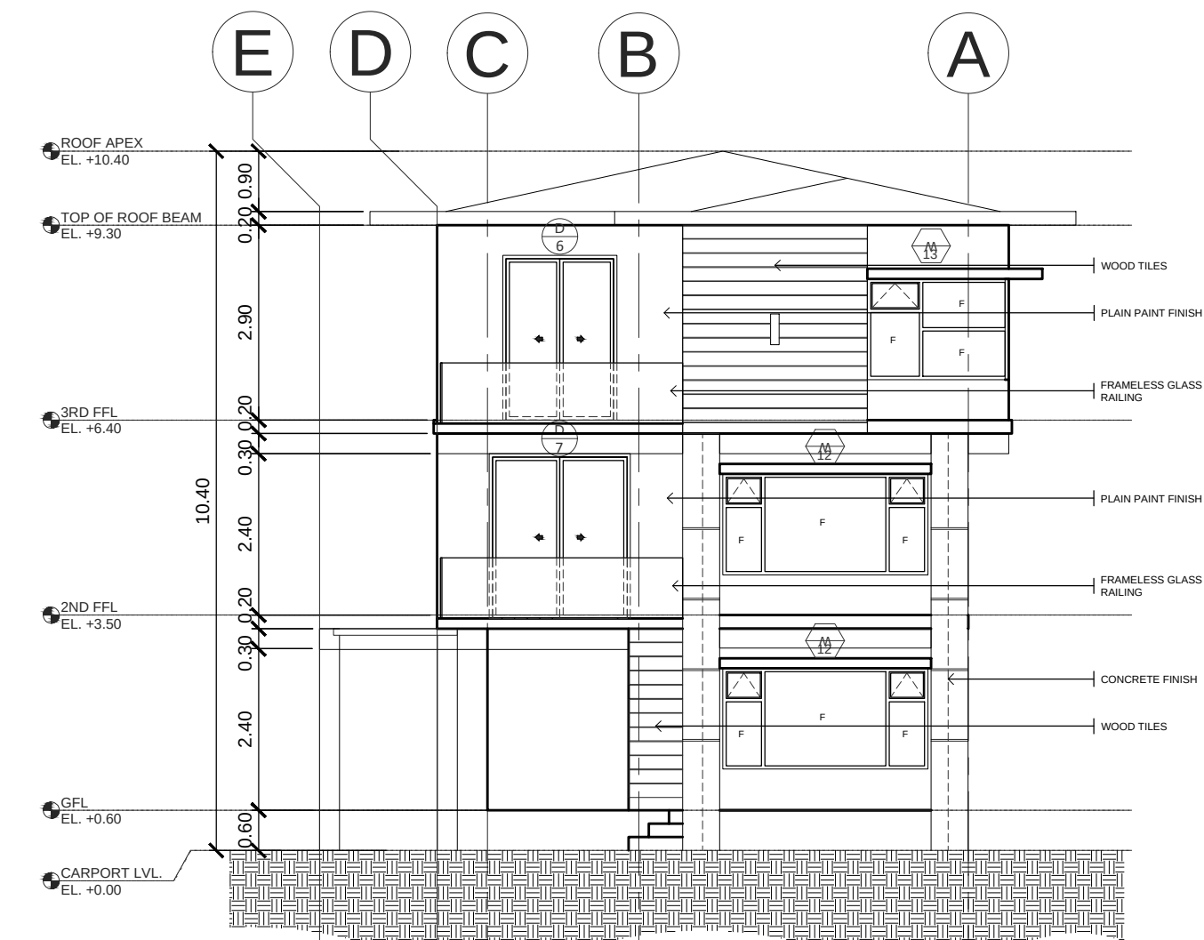
ARANETA RESIDENCE 3 FRONT ELEVATION A-06 SCALE: 1:100 MTS
