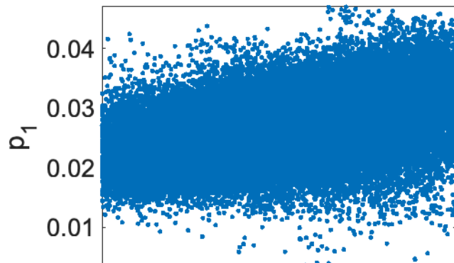
MIC
