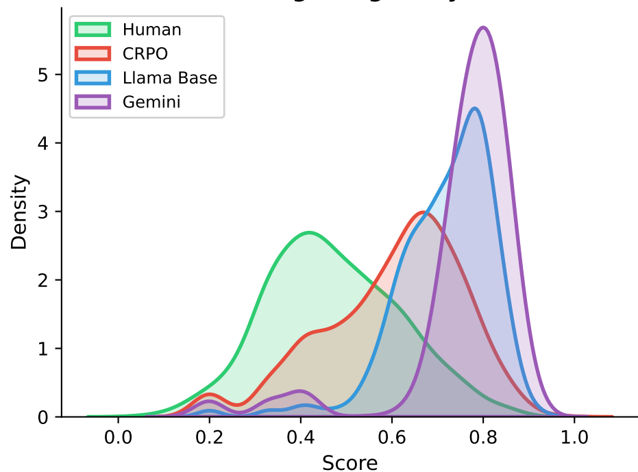
Story Creativity (MAoSS)
