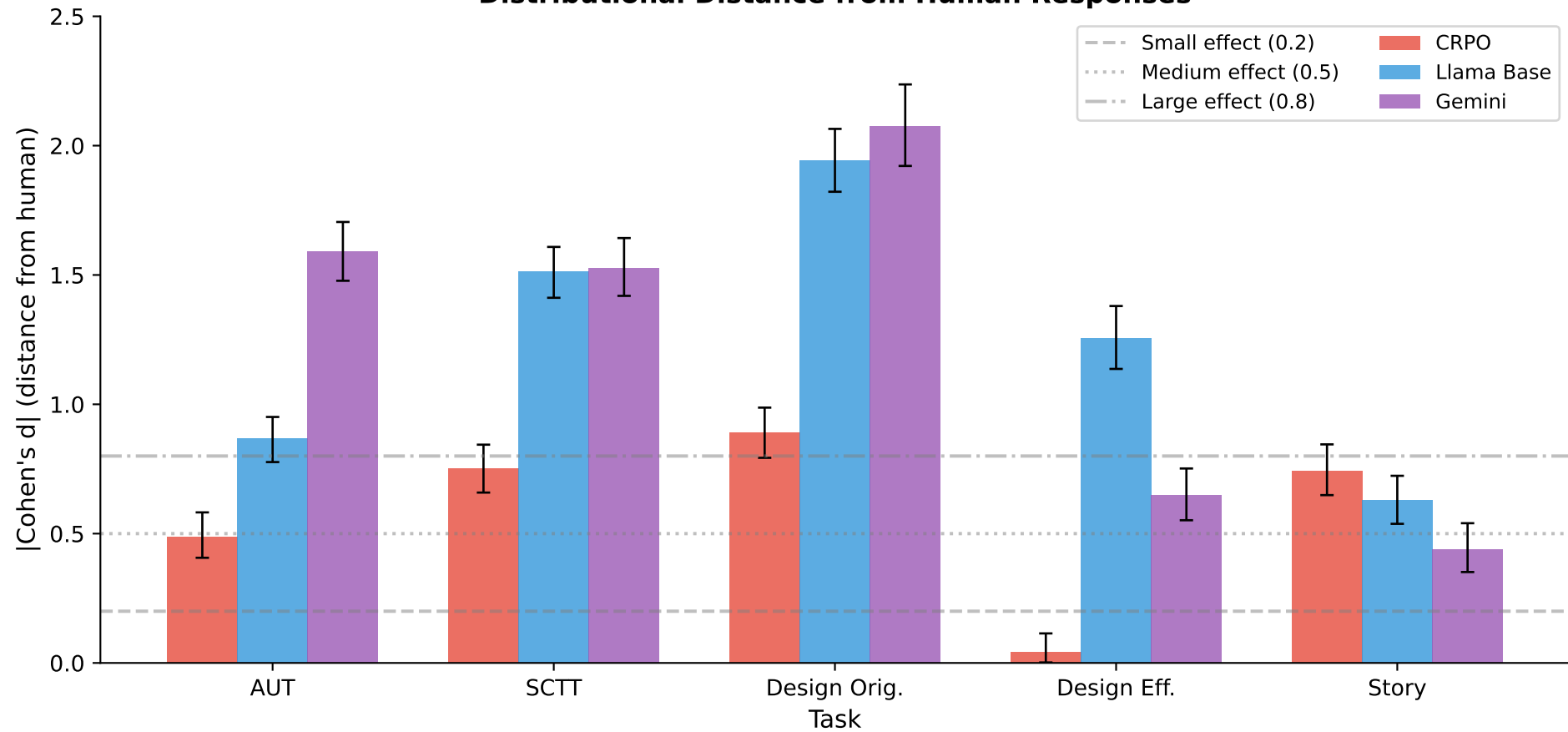
Distributional Distance from Human Responses
