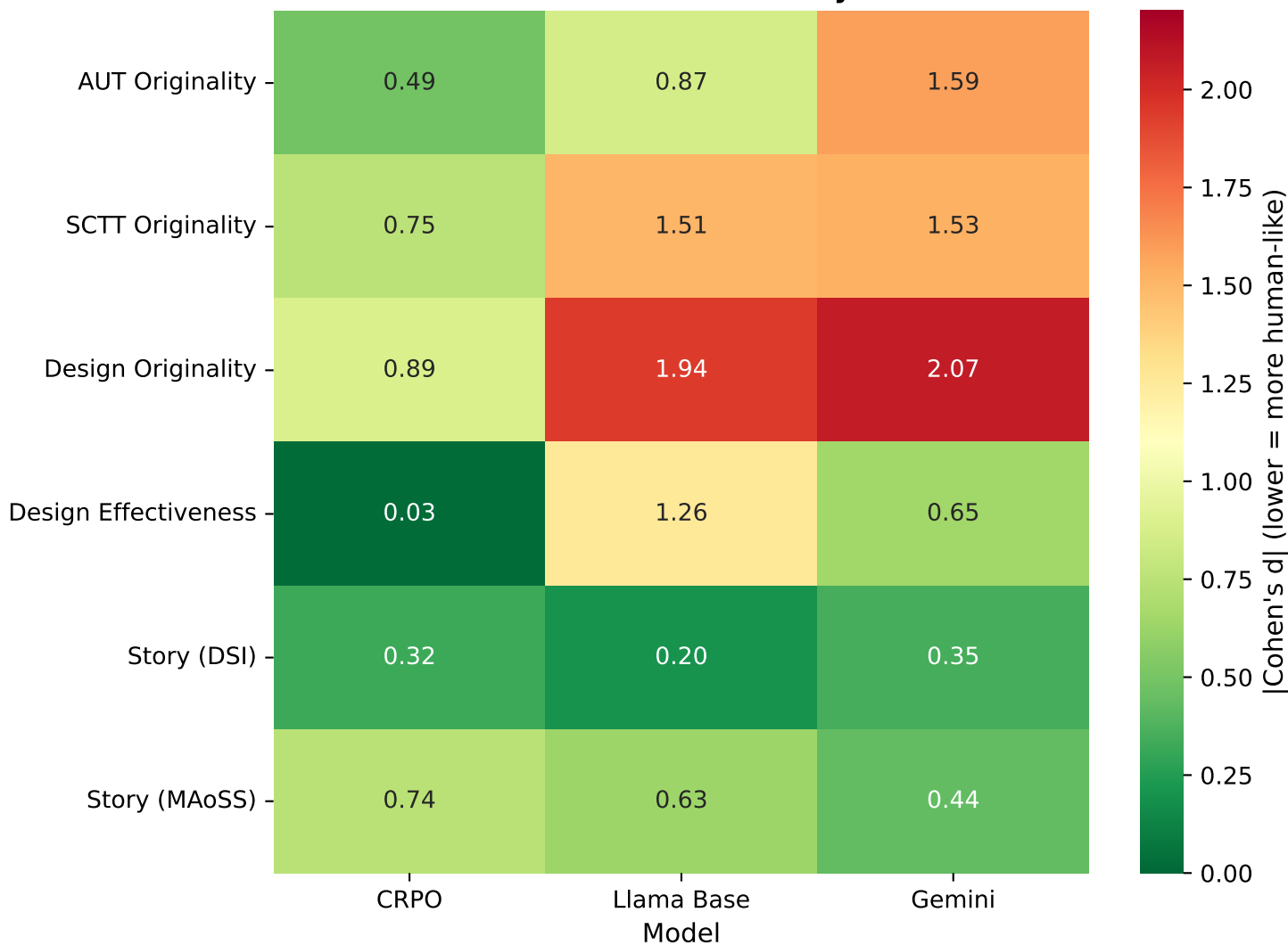
Distance from Human Distribution by Task and Model
