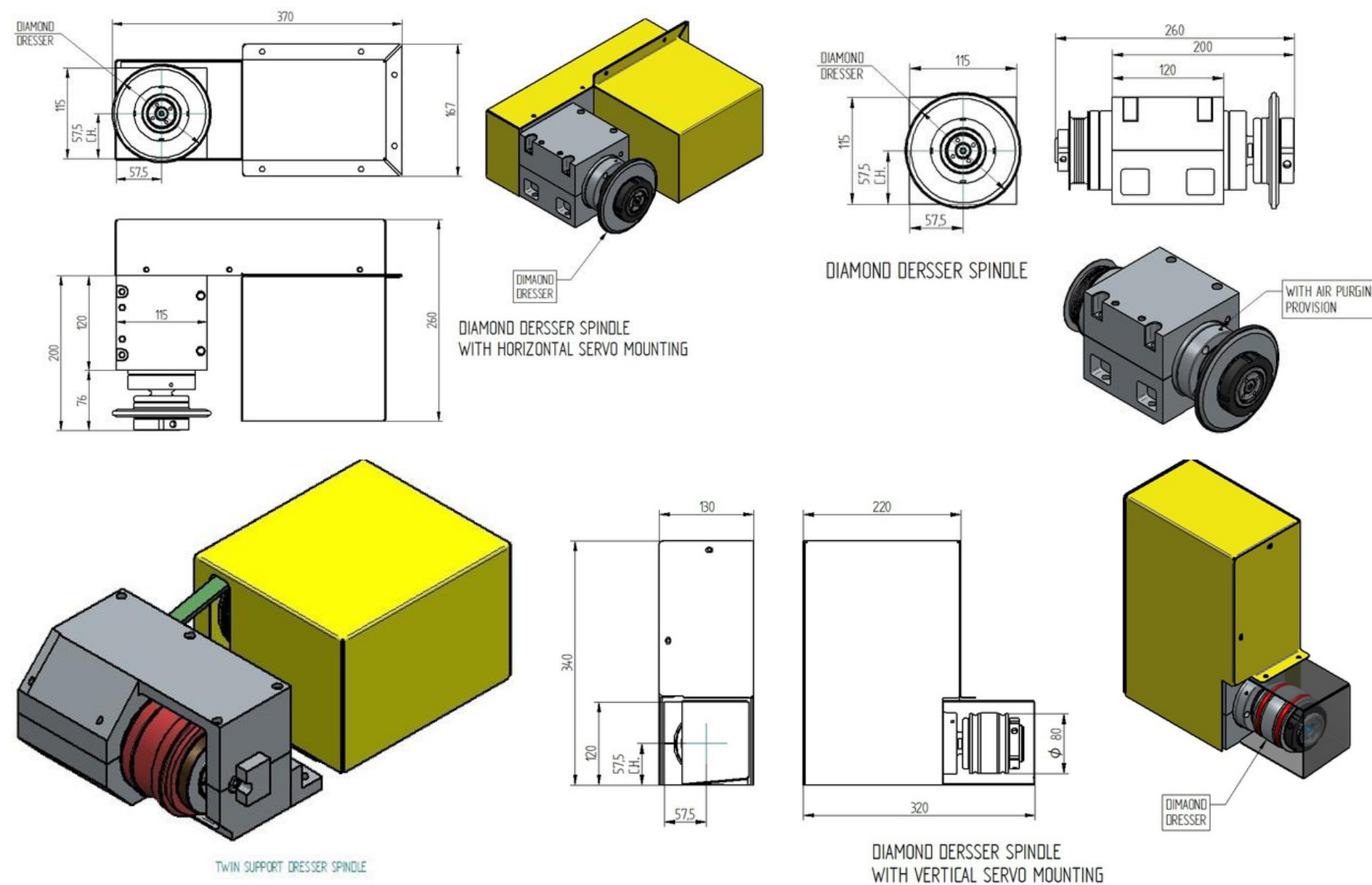
Dressing Spindle
