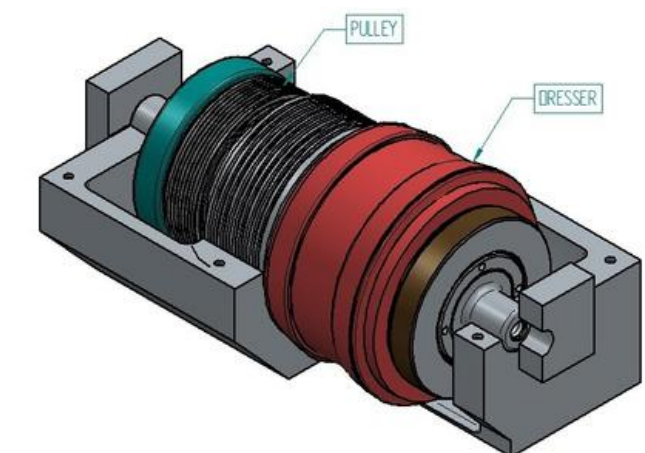
TWIN SUPPORT DRESSER SPINDLE
