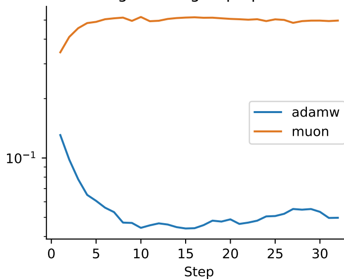
Matching matrix-group update norm
