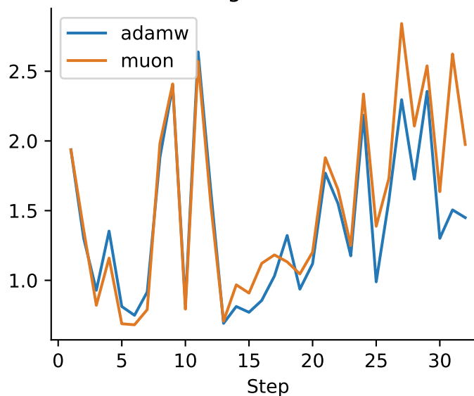
Matching matrix-group update norm
