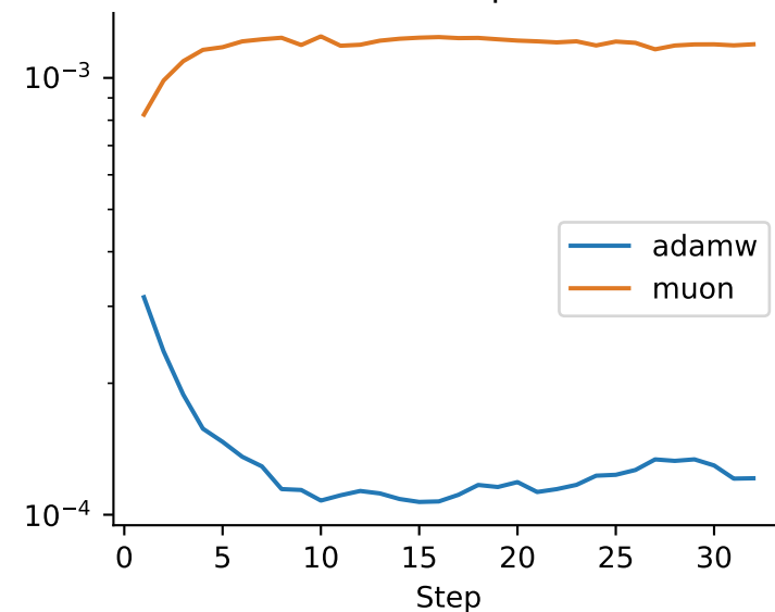
Fallback-group update norm
