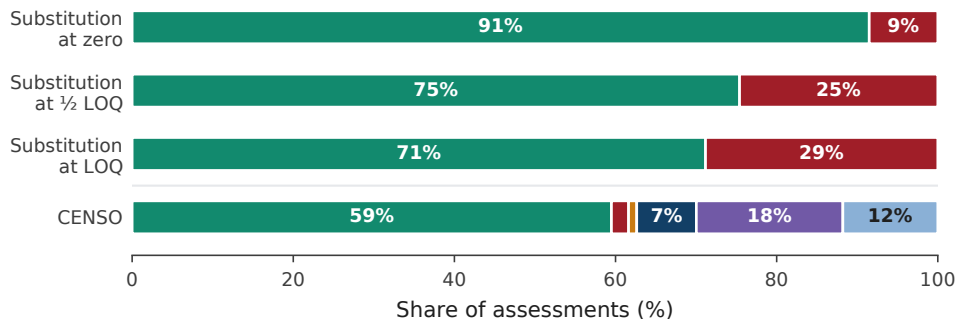
(a) The same 696,168 assessments, read four ways Substitution reports 59,251–200,708 exceedances; 14,809 are affirmed
