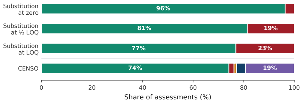
(b) The last five years only, 264,135 assessments The method fails the standard in 19% against 18% above, and no bound is missing
