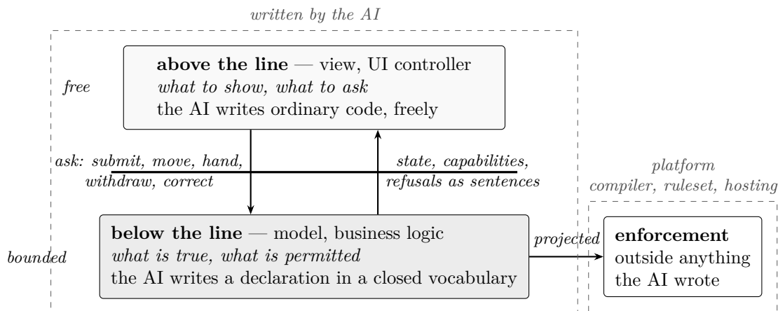
Figure 1: The line. The AI’s freedom differs on the two sides. The page above can only ask, through five intents; the declaration below decides, and it decides through enforcement that neither the page nor the AI can bypass.
