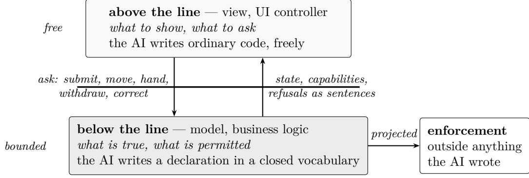
Figure 1: The line. The AI’s freedom differs on the two sides. The page above can only ask, through five intents; the declaration below decides, and it decides through enforcement that neither the page nor the AI can bypass.
