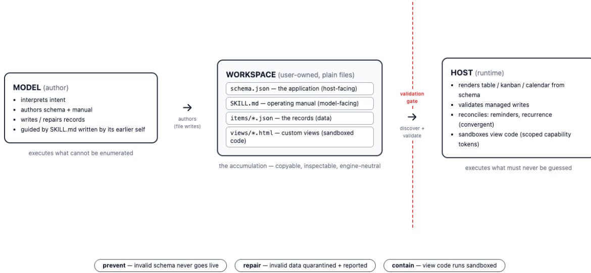
Figure 1: The schema-as-application architecture. The model authors declarative artifacts into the plain-file workspace; a validation gate ensures an invalid schema never becomes a live application; the host runtime—not the model—renders, validates, and reconciles over the user-owned records. Enforcement is tiered by consequence: prevent (applications), repair (data), contain (code).
