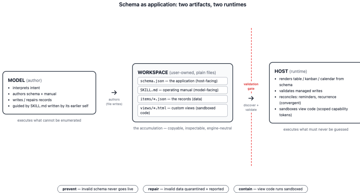
Figure 1: The schema-as-application architecture. The model authors declarative artifacts into the plain-file workspace; a validation gate ensures an invalid schema never becomes a live application; the host runtime—not the model—renders, validates, and reconciles over the user-owned records. Enforcement is tiered by consequence: prevent (applications), repair (data), contain (code).
