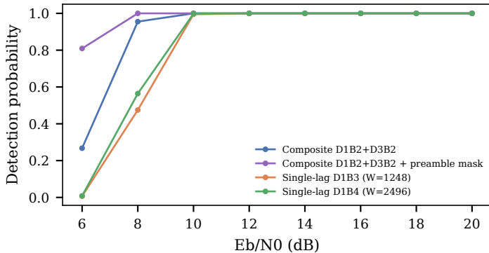
(a) Detection
