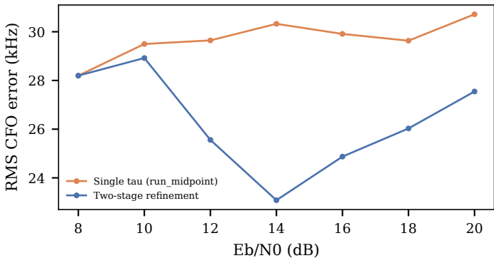
(b) CFO estimation accuracy
