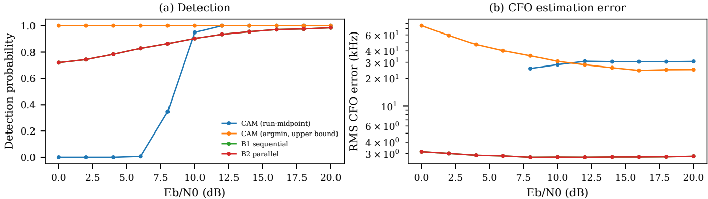
Fig. 4: Performance vs. SNR ( \ell=142 , w=624 )
