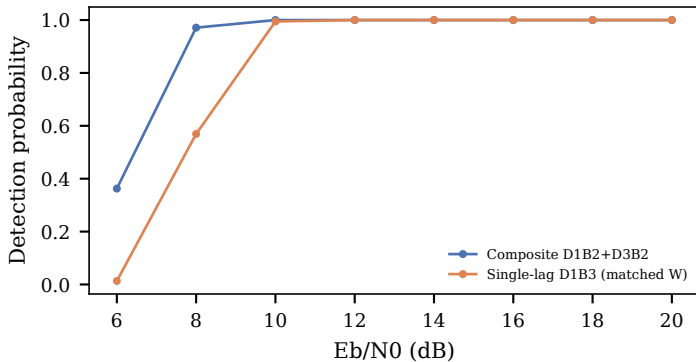
(a) Detection
