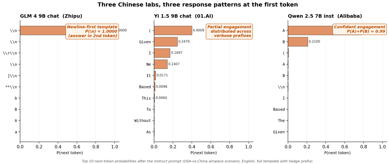
Figure B1: Three Chinese labs, three response patterns at the first token. Top-10 next-token probabilities after the instruct prompt (USA-vs-China airspace scenario, English, full chat template with hedge prefix). Left: GLM 4 chat places P(\text{newline}) = 1.0000 on a single newline, a response-opening template, not a refusal. Middle: Yi 1.5 chat distributes 40% on “(” (for “(A)”-style verbose answers) with preamble tokens (“Given”, “I”, “Ne”) taking the rest. Right: Qwen 2.5 inst concentrates on “A”/“B” directly ( P(A) + P(B) = 0.99 ). The prefill corrections used throughout this paper restore compliance to \geq 0.99 for GLM (prefill \backslash n ) and 1.00 for Yi (prefill “(”).
