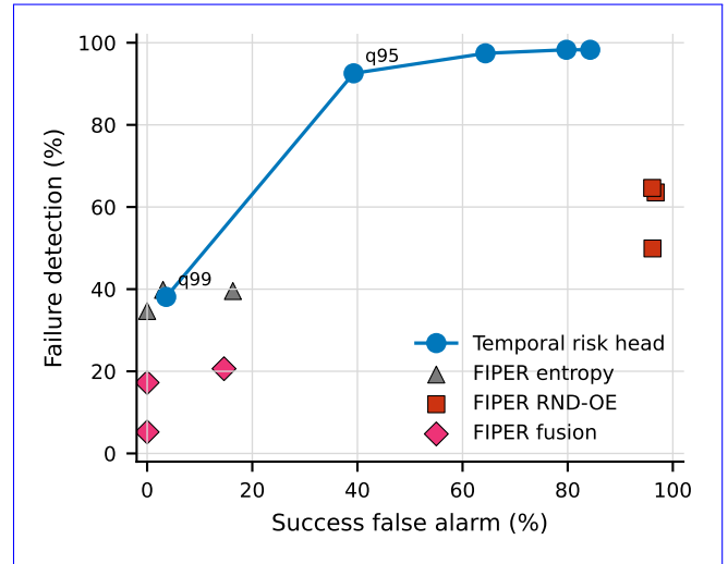
Fig. 3. Seen-calibrated monitor transfer to six unseen suites. Each point is computed on the same 331 successful and 349 failed episodes. The temporal risk-head curve varies only thresholds fixed on seen data; the three points per FIPER family are its CT-quantile, TVT-quantile and TVT-CP-band rules. Neither method is recalibrated on the OOD outcomes.
