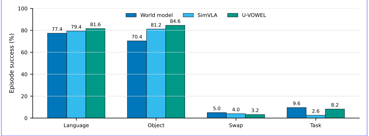
Fig. 4. Suite-level success on matched official LIBERO-PRO episodes. The selected U-VOWEL controller improves the aggregate result through the Language and Object suites, but does not solve the Swap or Task shifts.
