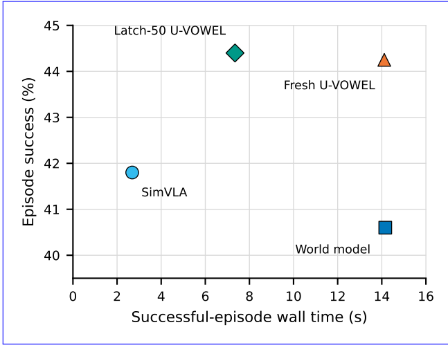
Fig. 5. Official LIBERO-PRO success versus measured wall time on successful episodes. The latch improves the compute profile of fresh routing without a measurable success difference on the matched manifest.
