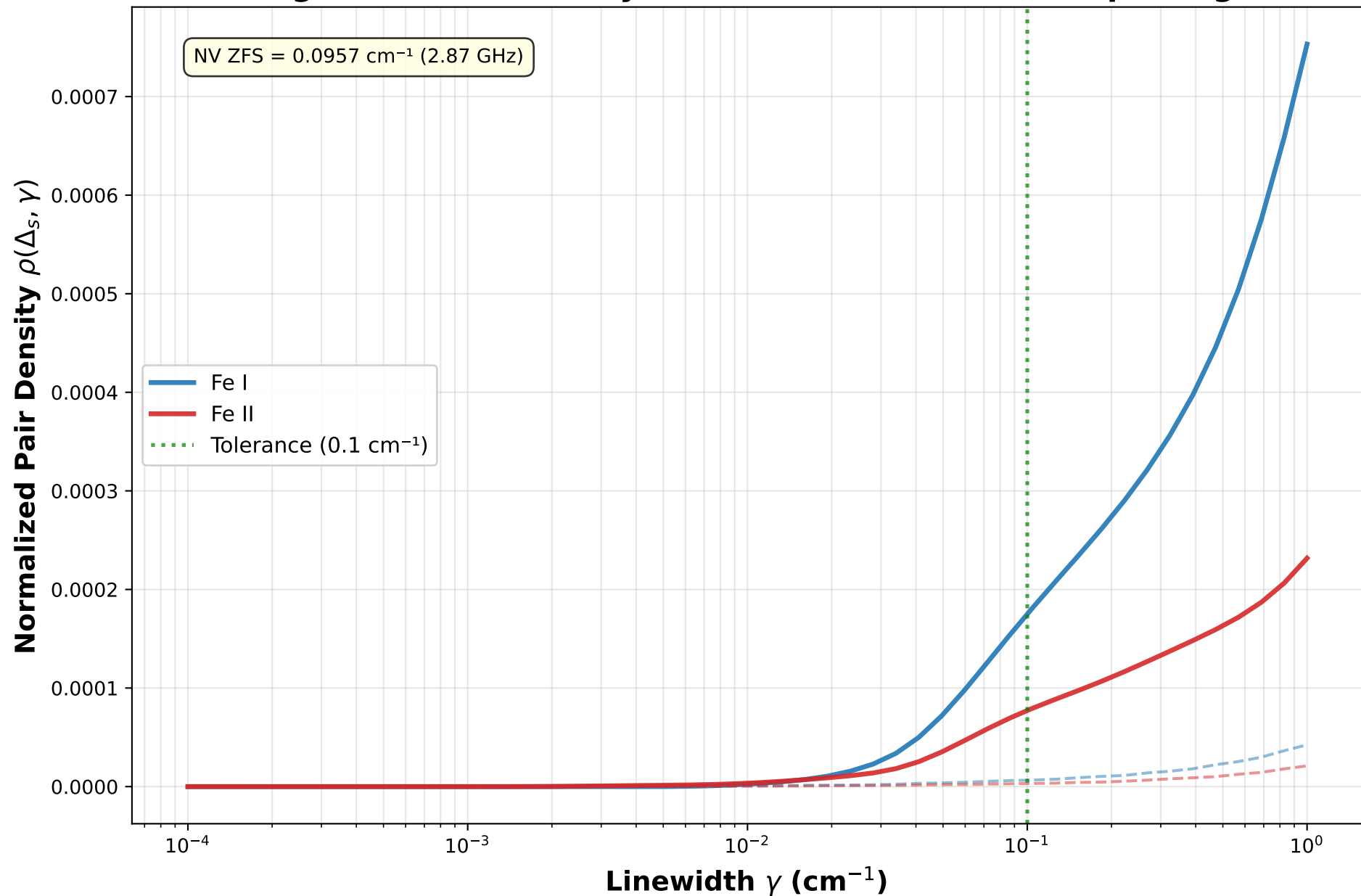
Figure 1: Pair Density Scan near NV Zero-Field Splitting
