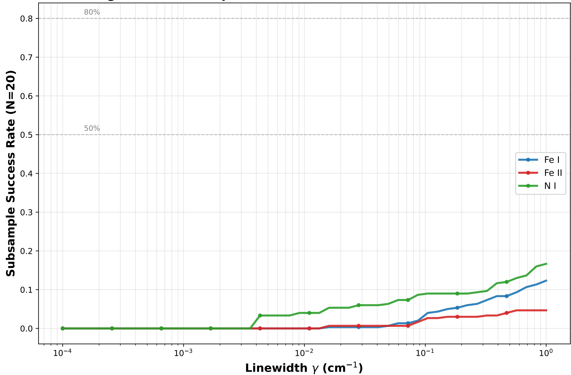
Figure 2: Subsample Robustness of Raman Pair Detection
