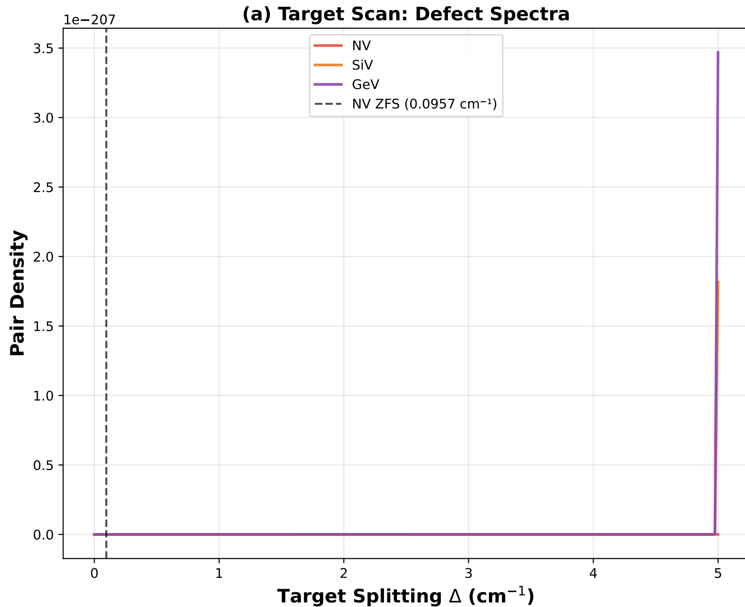
Figure 3: Defect Spectra — Absence of Raman Pairs near NV ZFS
