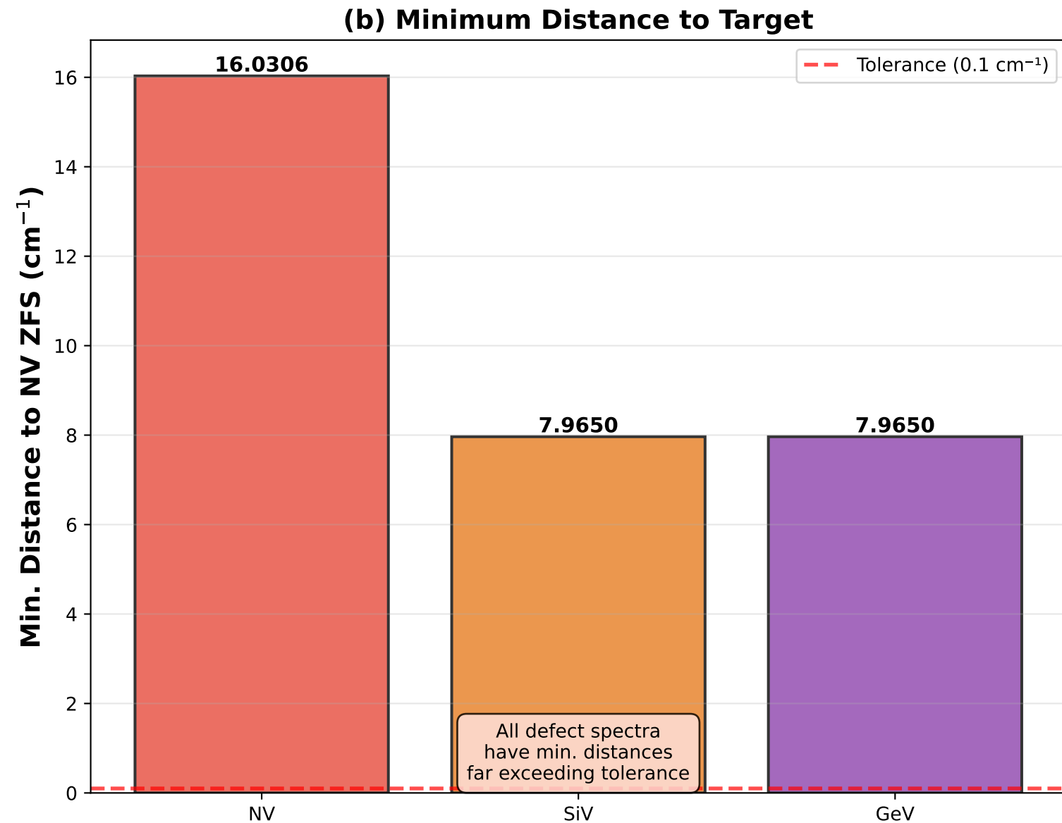
Figure 3: Defect Spectra — Absence of Raman Pairs near NV ZFS
