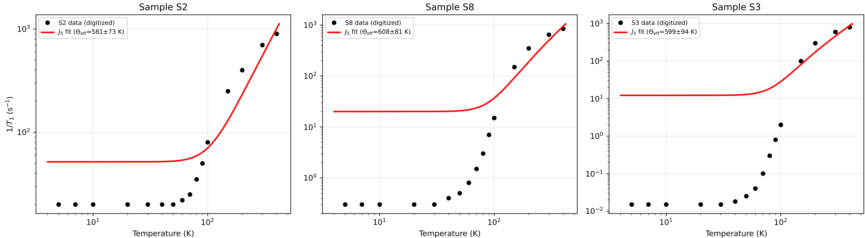
Figure 1: J_5 transport fits to Jarmola et al. (2012) using fixed Table 1 \Theta_{\text{eff}} values
