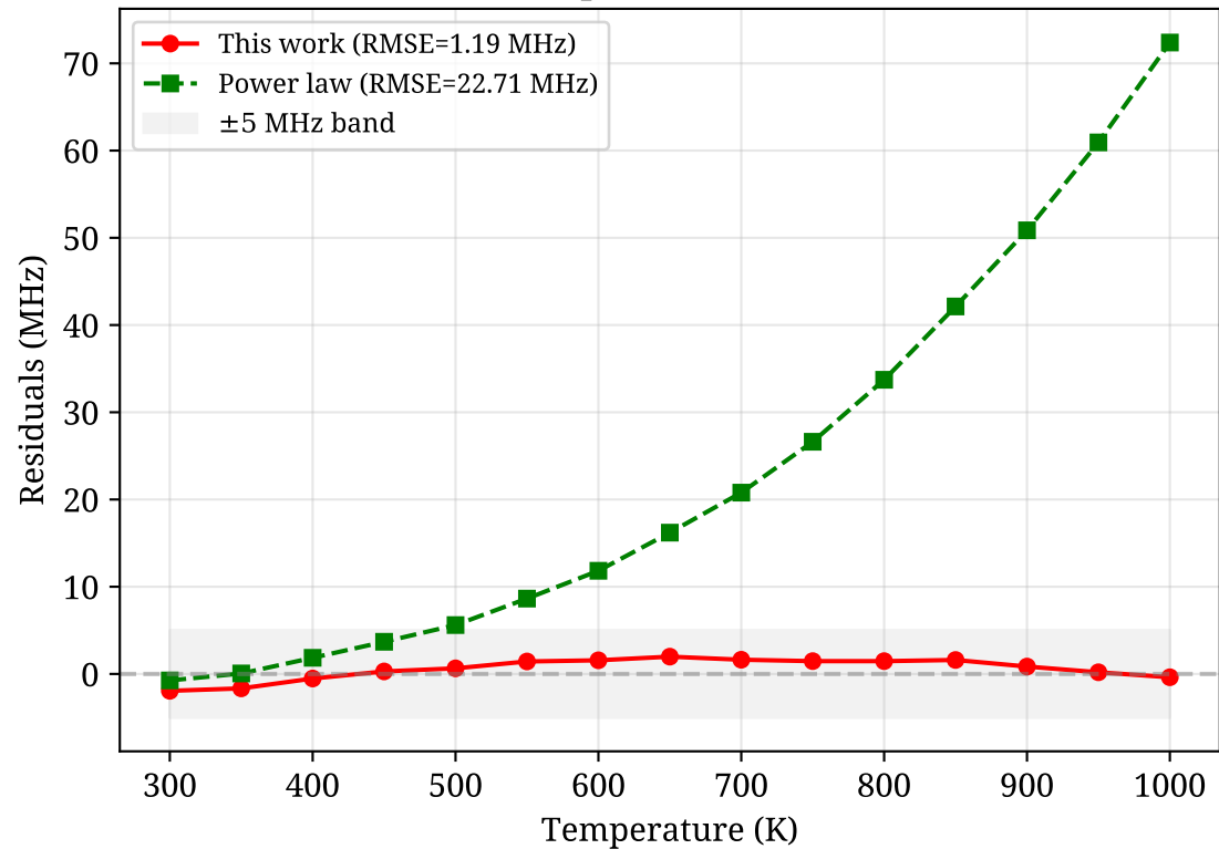
(b) Extrapolation Residuals
