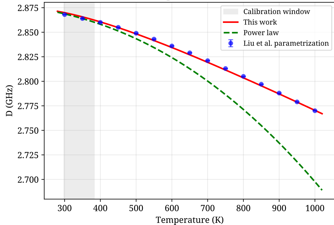
(a) Extrapolation to 1000 K
