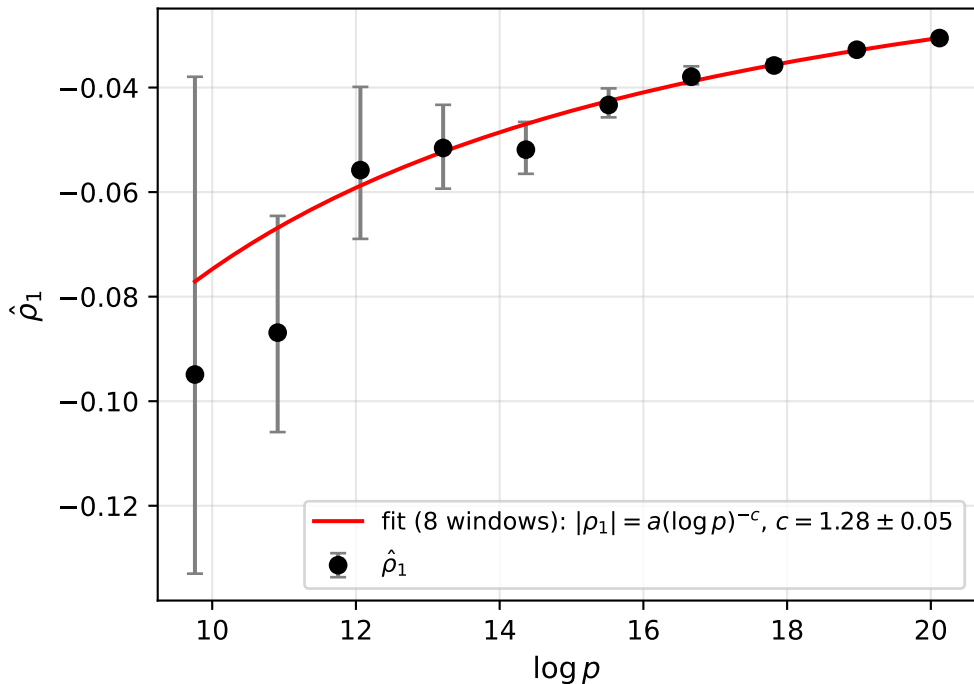
Lag-one autocorrelation across logarithmic windows
