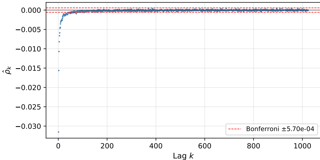
Detrended ( \delta_n ) correlogram, K = 1024 — 255/1024 positive
