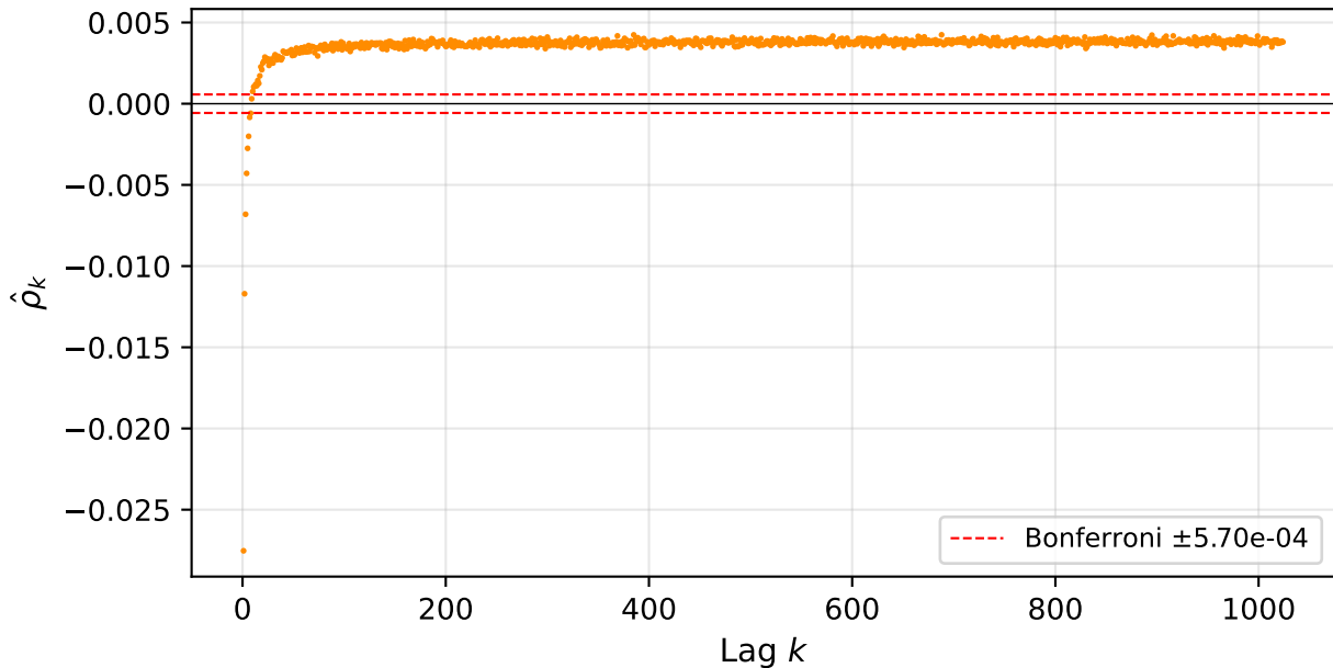
Raw ( g_n ) correlogram, K = 1024 — 1016/1024 positive (artifact)
