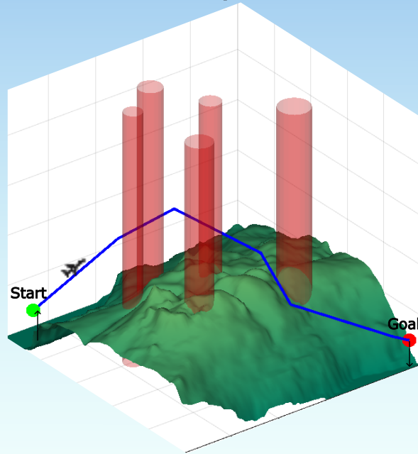
3D UAV Flight Planning from Algorithm
