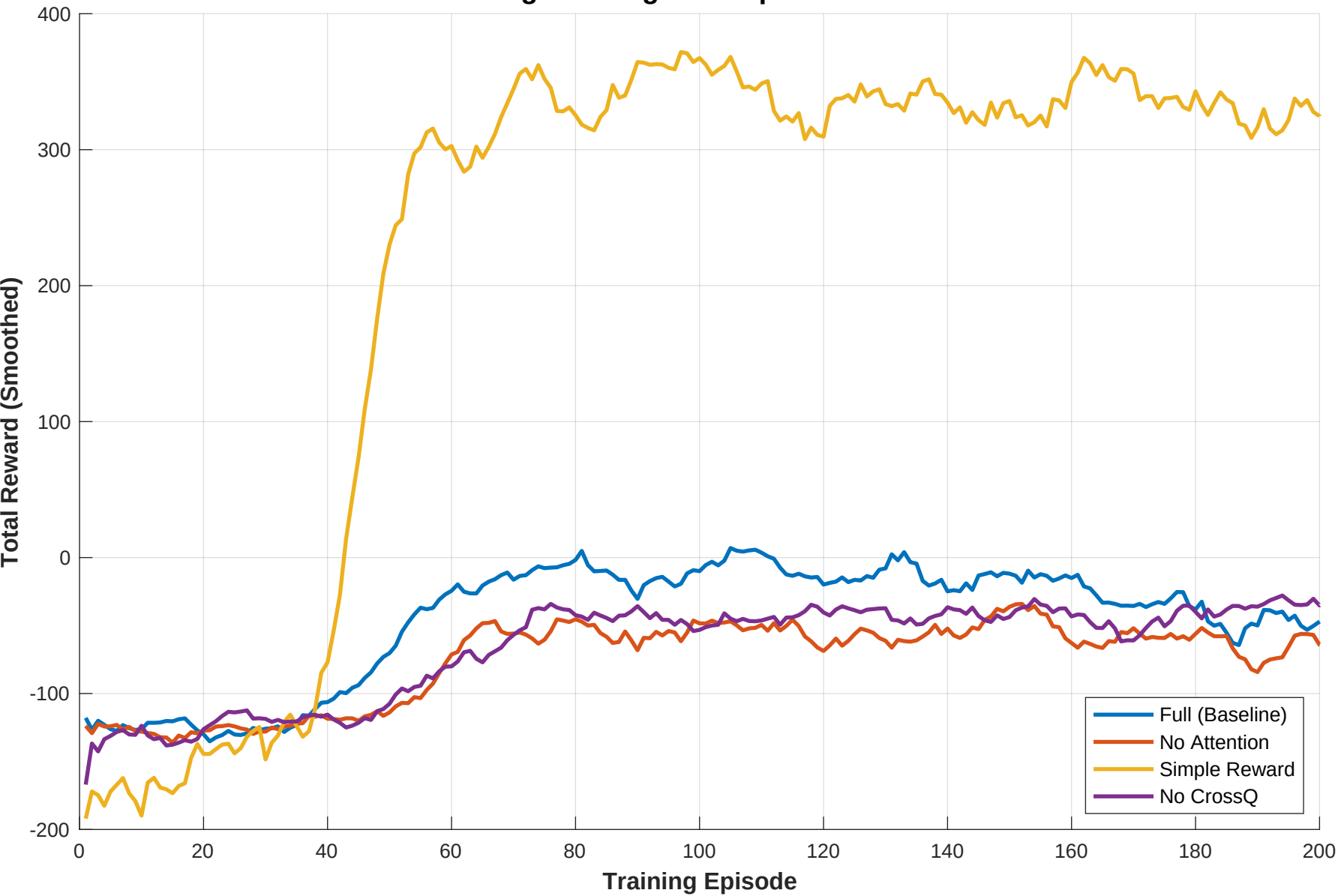
Training Convergence: Episode Rewards
