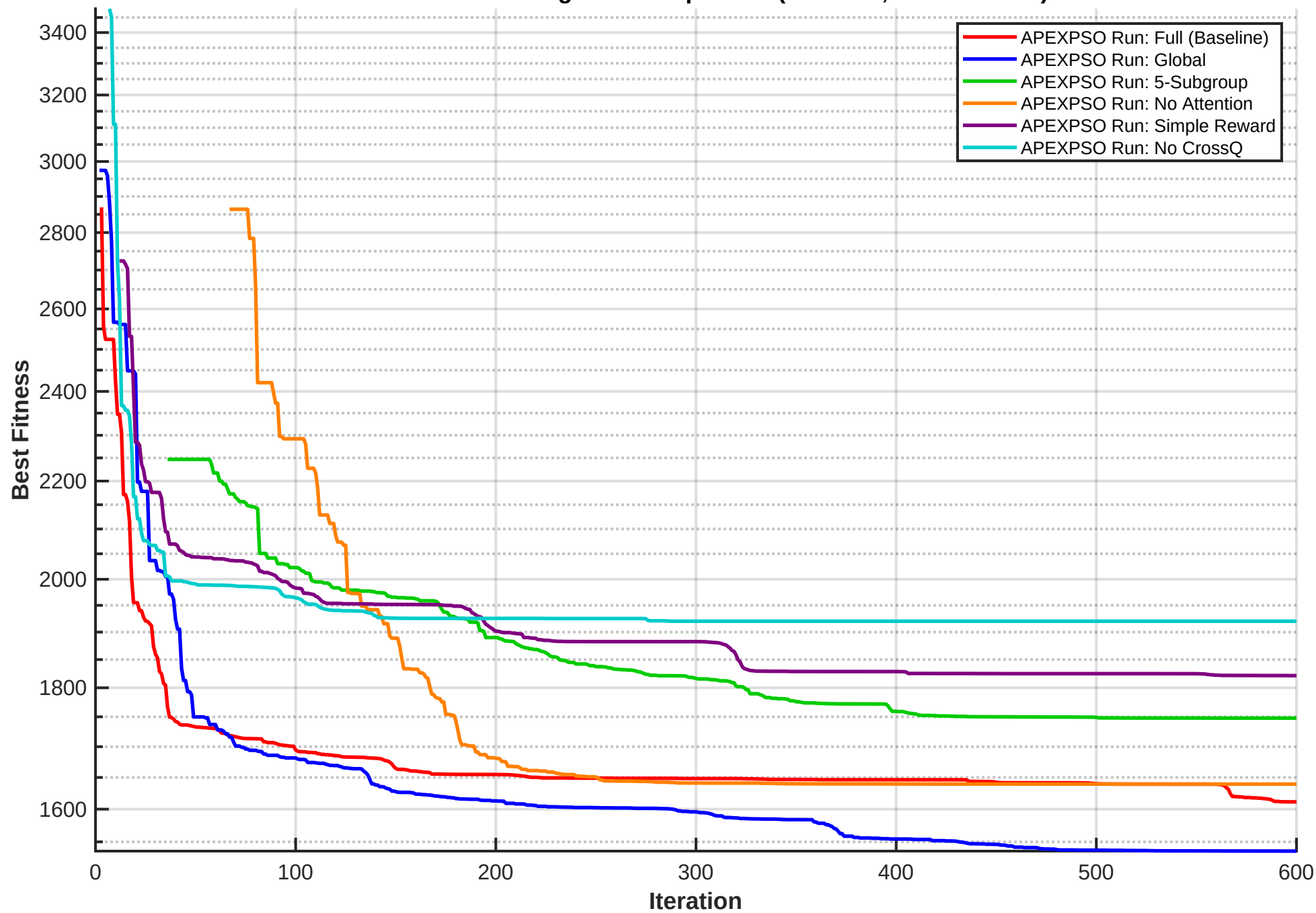
Scenario 1: Convergence Comparison (30 Trees, 30 Obstacles)
