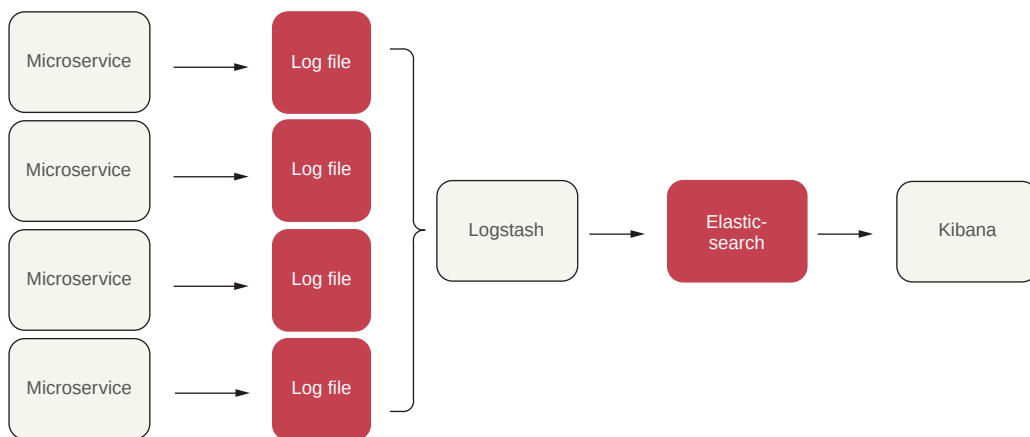
Figure 2.11 Managing the microservice logs with the ELK architecture
