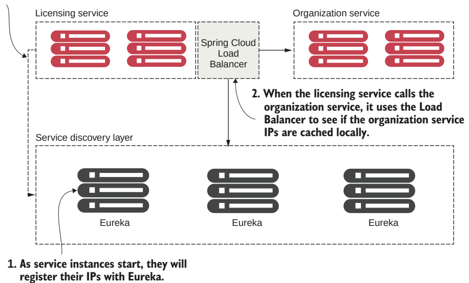
Figure 6.4 By implementing client-side caching and Eureka with O-stock's licensing and organization services, you can lessen the load on the Eureka Servers and improve client stability if Eureka becomes unavailable.
