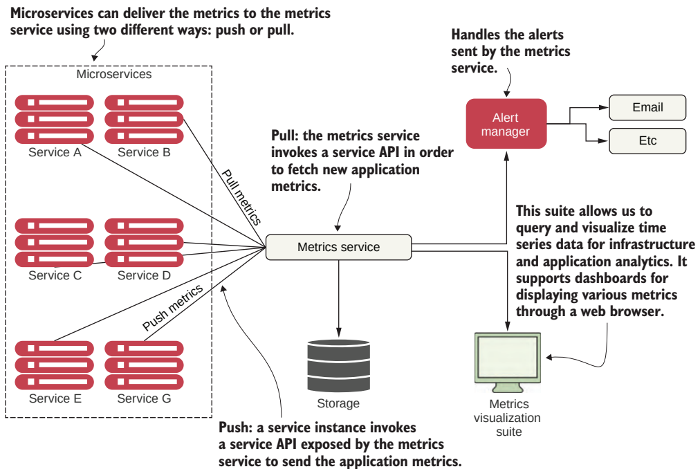
Figure 1.16 Metrics are pulled or pushed from the microservices and collected and stored in the metrics service to be shown using a metrics visualization suite and an alert management tool.
