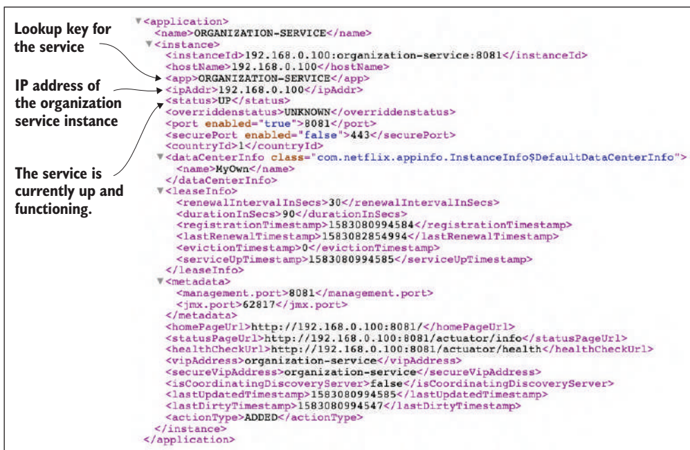
Figure 6.6 The Eureka REST API showing the organization service. The response shows the IP address of the service instances registered in Eureka, along with the service status.
