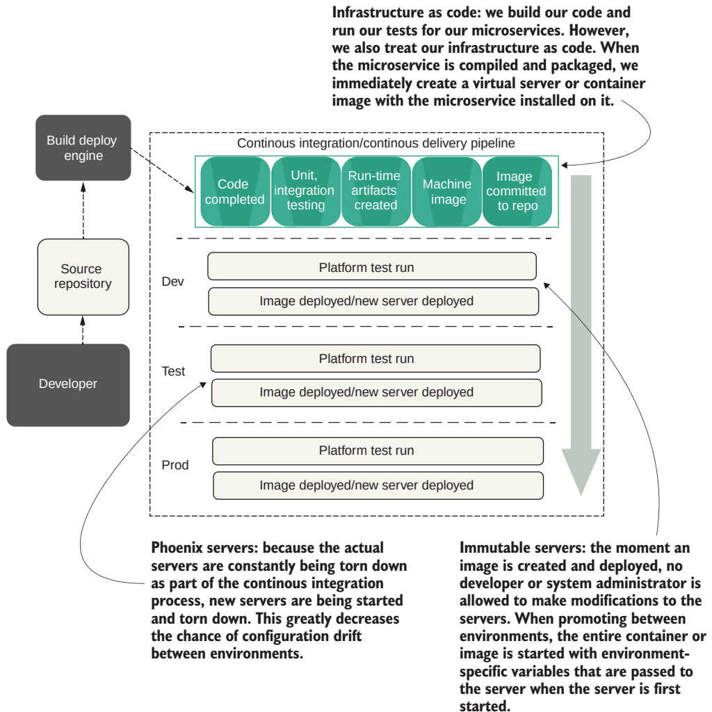
Figure 1.17 You want the deployment of the microservice and the server it's running on to be one atomic artifact that's deployed as a whole between environments.
