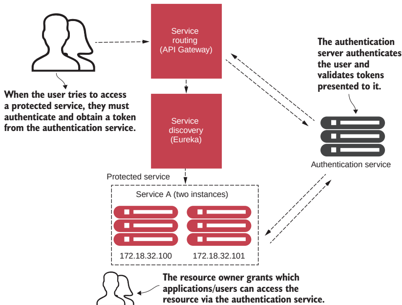
Figure 1.14 Using a token-based security scheme, you can implement service authentication and authorization without passing around client credentials.
