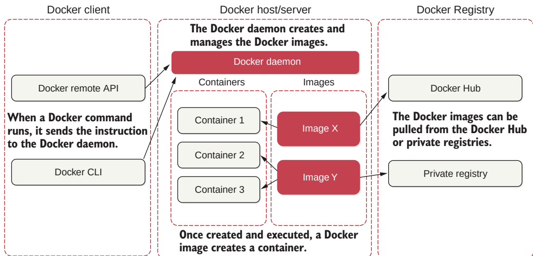
Figure 4.2 Docker architecture composed of the Docker client, the Docker host, and the Docker Registry.
