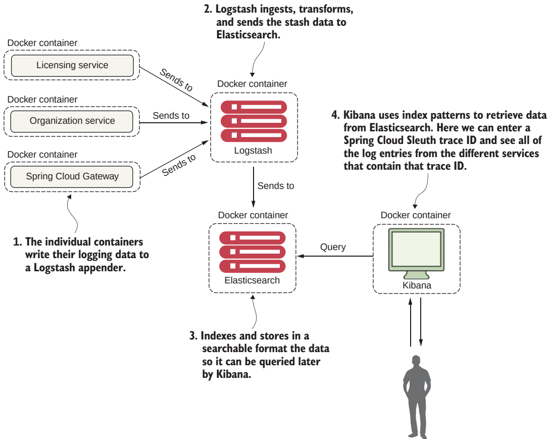
Figure 11.4 The ELK Stack allows us to quickly implement a unified logging architecture.
