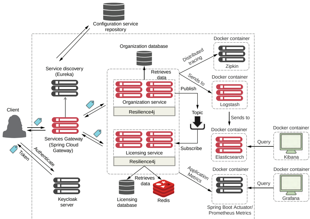
Figure 1.4 High-level overview of the services and technologies that we'll use in this book
