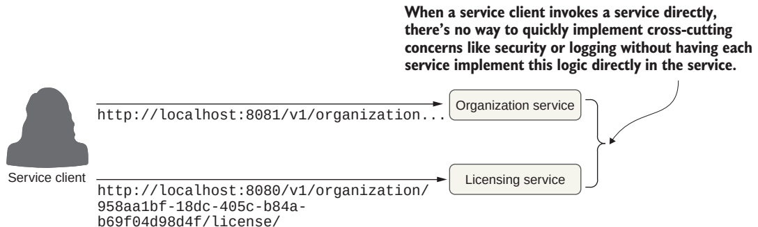
Figure 8.1 Without a service gateway, the service client calls distinct endpoints for each service.
