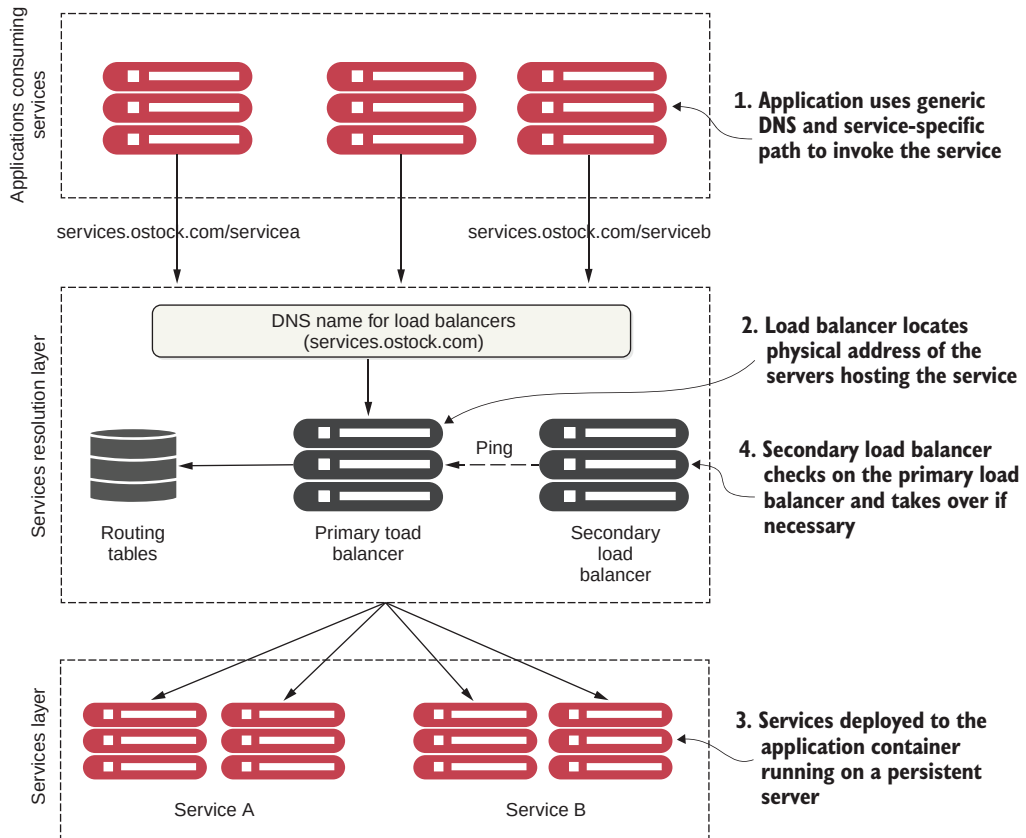
Figure 6.1 A traditional service location resolution model uses a DNS and a load balancer.
