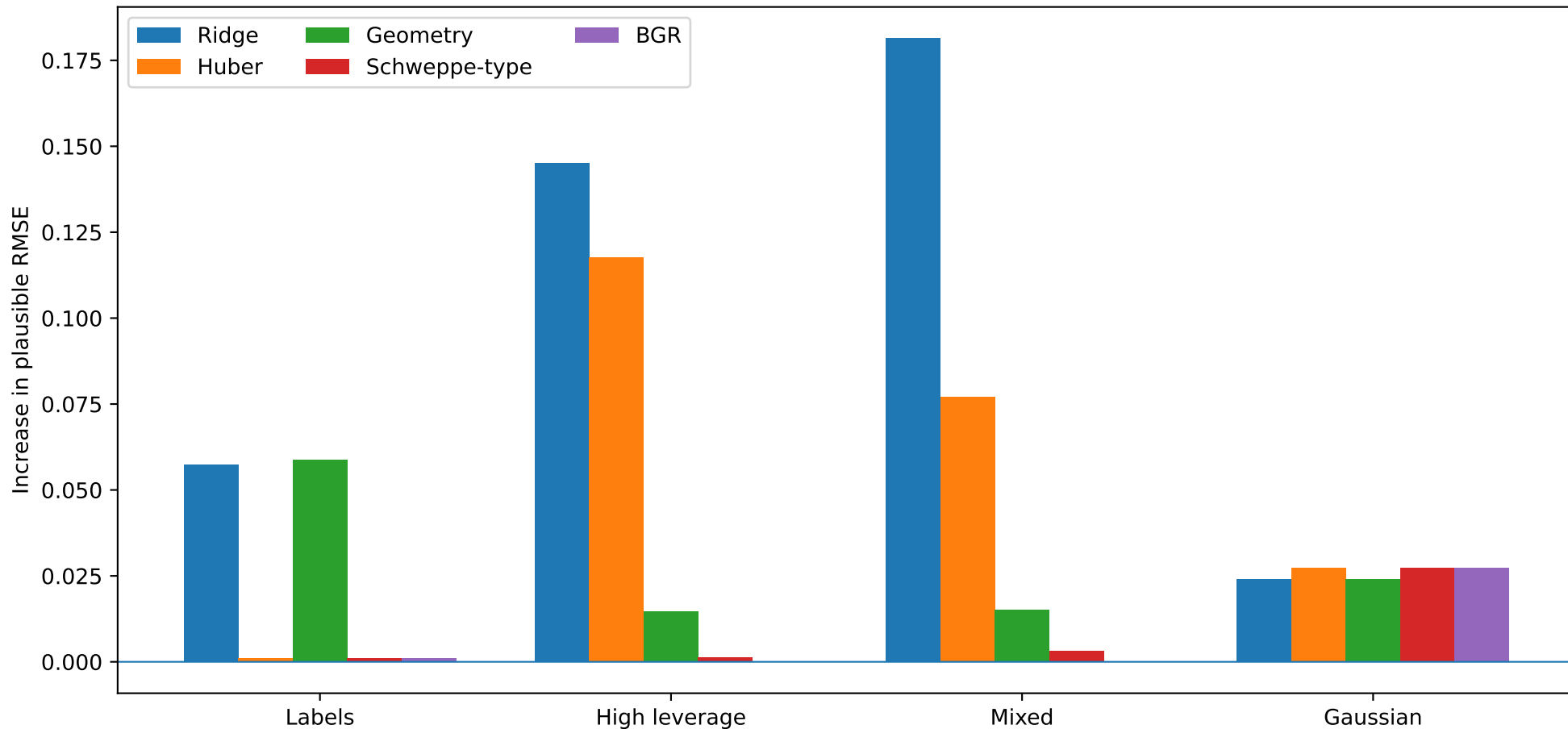
SeLogger: degradation under contamination (internal evaluation holdout)
