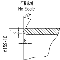
N5~6/N7~8接管详图 NOZZLE N5~6/N7~8 DETAIL
