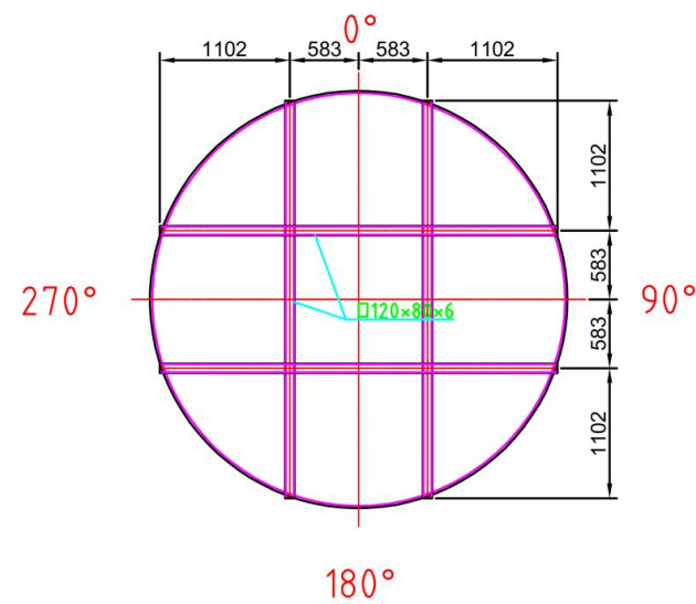
Layout plan for strengthening the roof
