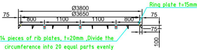
A-A Ring plate layout drawing
