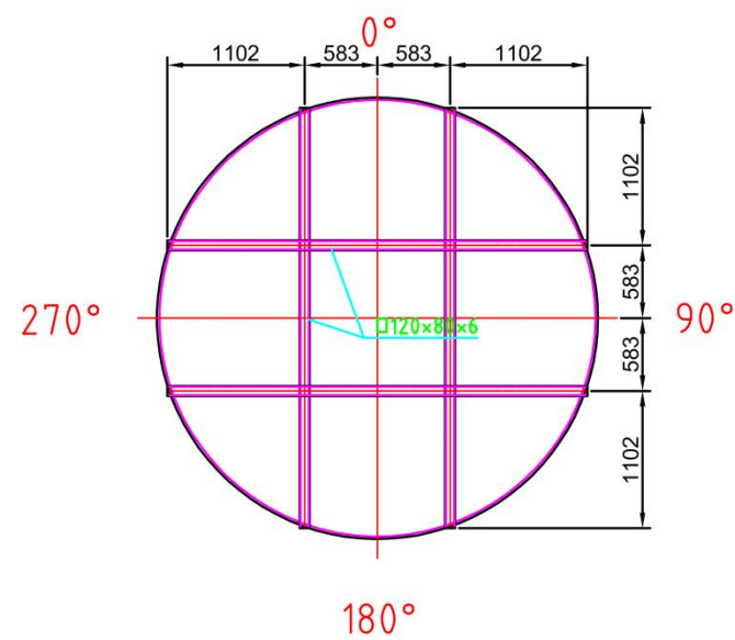
Layout plan for strengthening the roof
