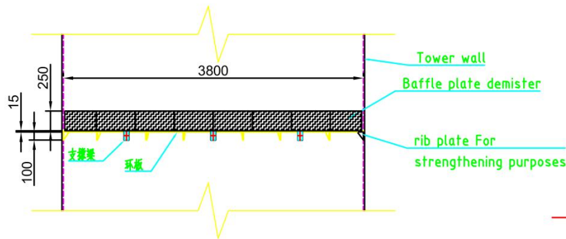
Elevation layout of demister
