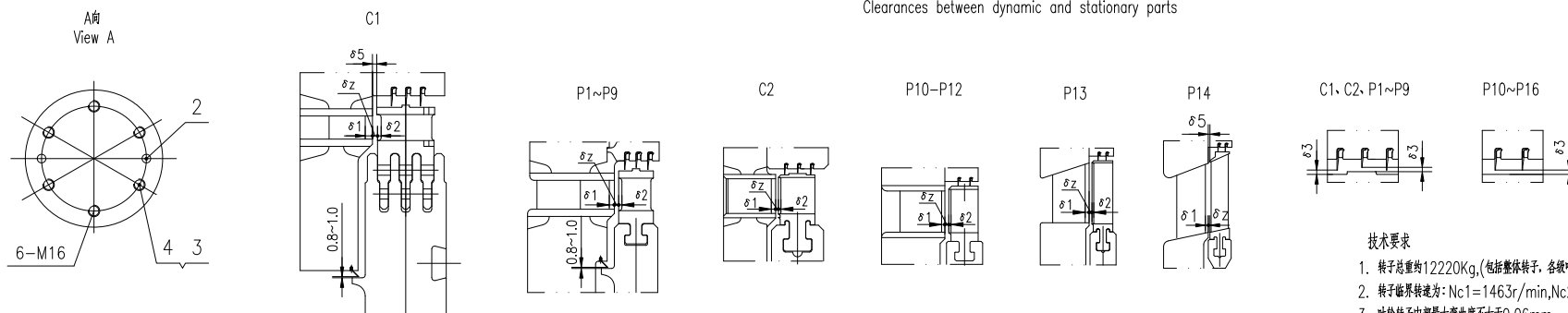
动静间隙图 Clearances between dynamic and stationary parts
