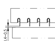
隔板汽封详图(P16-P17) Detail of diaphragm gland
