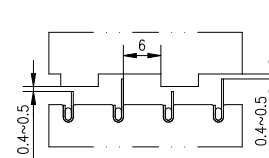
后汽封详图 Detail of rear gland
