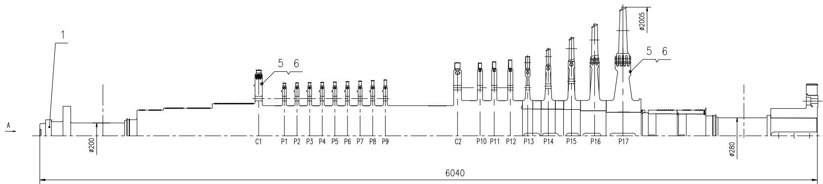
动静间隙图 Clearances between dynamic and stationary parts
