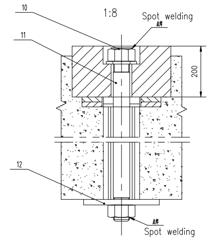
地脚螺栓安装示意图 Installation diagram of foundation bolt
