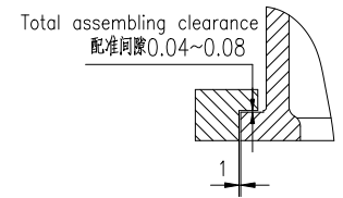
座架压板装配详图 Assembling detail of the pressure plate
