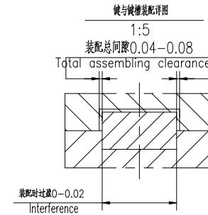
Assembly details of key and key way
