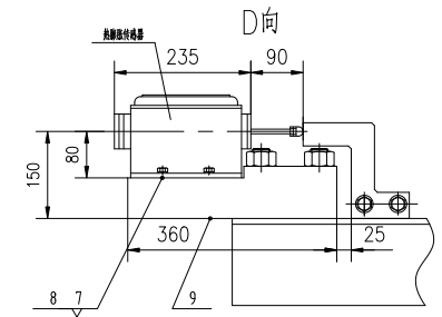
地脚螺栓安装示意图 Installation diagram of foundation bolt
