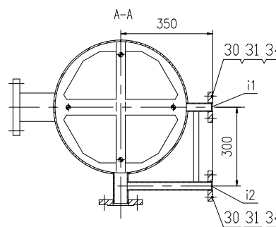
NOTES: 1.Model:LQ-40. 2.Cooling water flow rate 55~75t/h. 3.Cooling surface area 40m 2 . 4.Condensate working pressure 1.5Mpa. 5.Pressure for hydrostatic test: 2.25MPa in water chamber.and 0.2MPa in steam chamber The test will be held for 10 minutes,during which no leakage is allowed. 6.Cleanliness condition conforms to JB/T4058-2017 Standard of Cleanliness for steam Turbines. 7.Each interface of this device is provided with counter flange.
