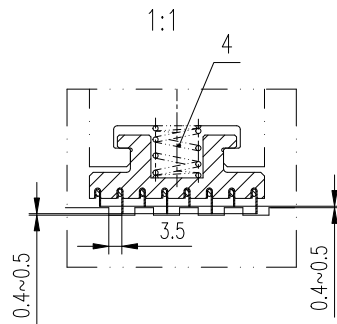
隔板汽封装配详图(C2、P1-P15) Assembling detail of Diaphragm gland
