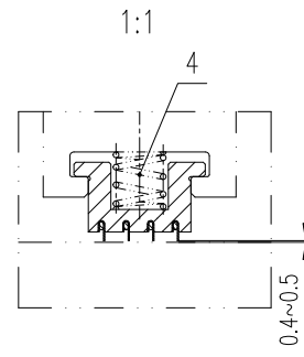
隔板汽封装配详图(P16-P17) Assembling detail of Diaphragm gland
