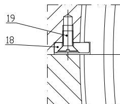
压板装配详图 Assembling details of pressure plate
