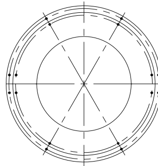
前汽封4段与汽缸装配间隙详图 Assembling details of 4th front gland
