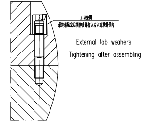
止动垫圈装配示意图 Assembling of external tab washers
