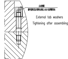
止动垫圈装配示意图 Assembling of external tab washers
