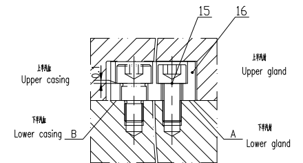
支撑板装配详图 Assembling details of support
