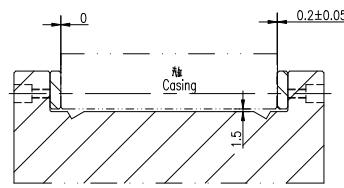
压板装配详图 Assembling details of pressure plate
