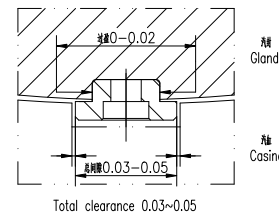
圆头键装配详图 Assembling details of round head key Total interference 0~0.02
